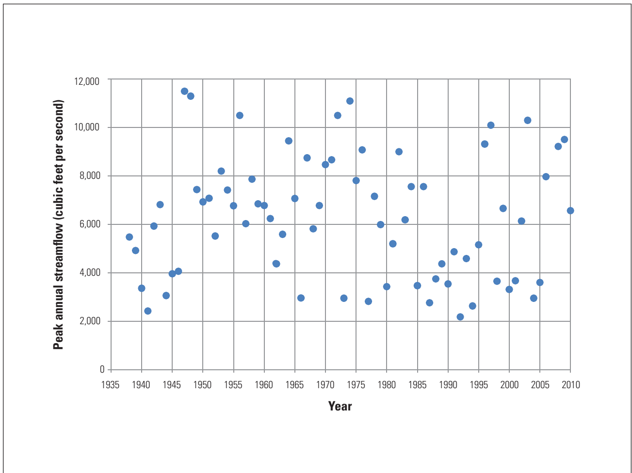
Figure 9. Bitterroot River streamflow near Darby, Montana (USGS 2011).
