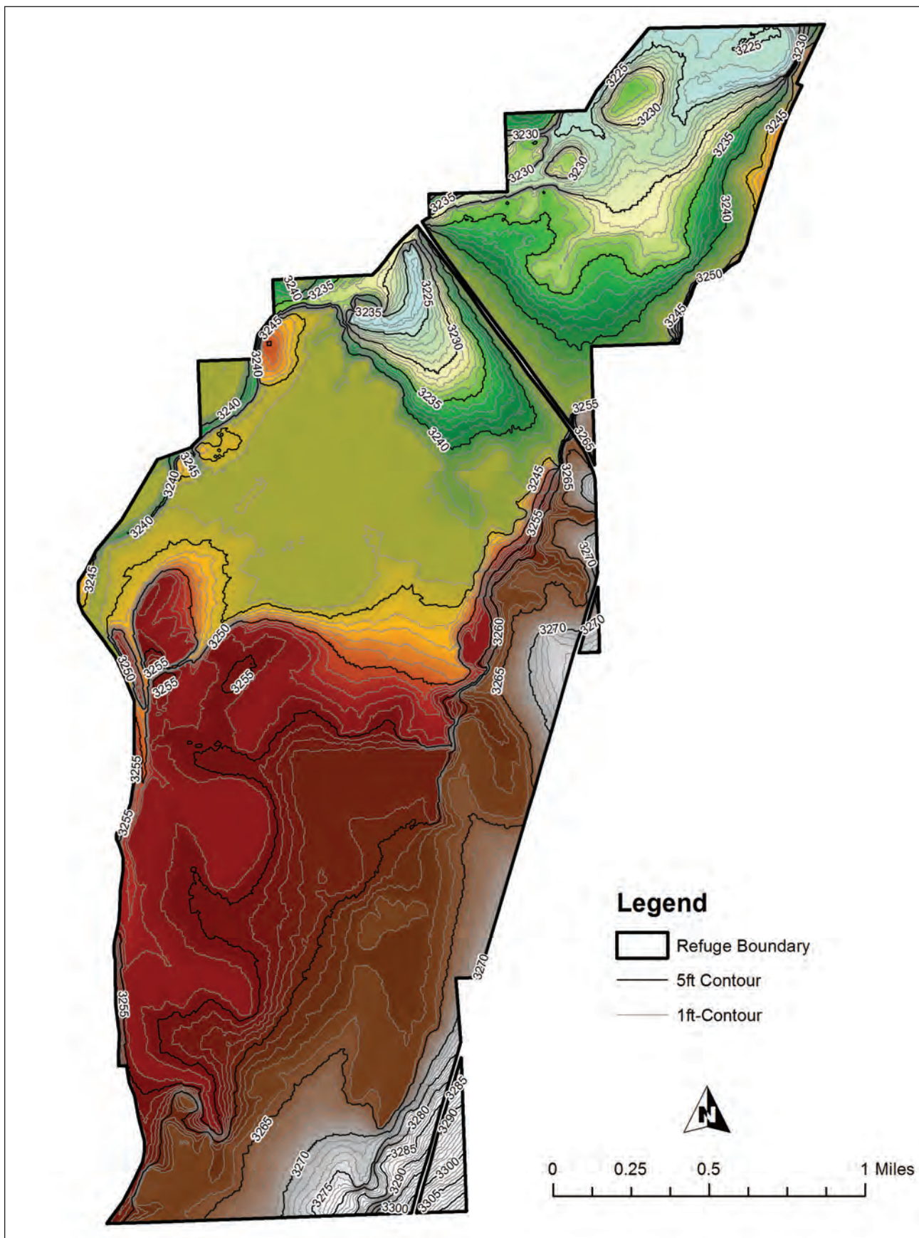
Figure 11. Map of Lee Metcalf National Wildlife Refuge, Montana, showing 1-foot contour intervals (Heitmeyer et al. 2010).
