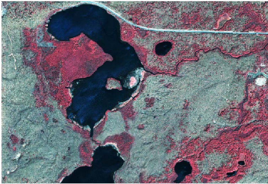
Figure 5 - Fine resolution imagery is the principle data source for determining wetland change. This example shows a false color infrared \leq 1 m resolution satellite image [Ikonos, 2005].
