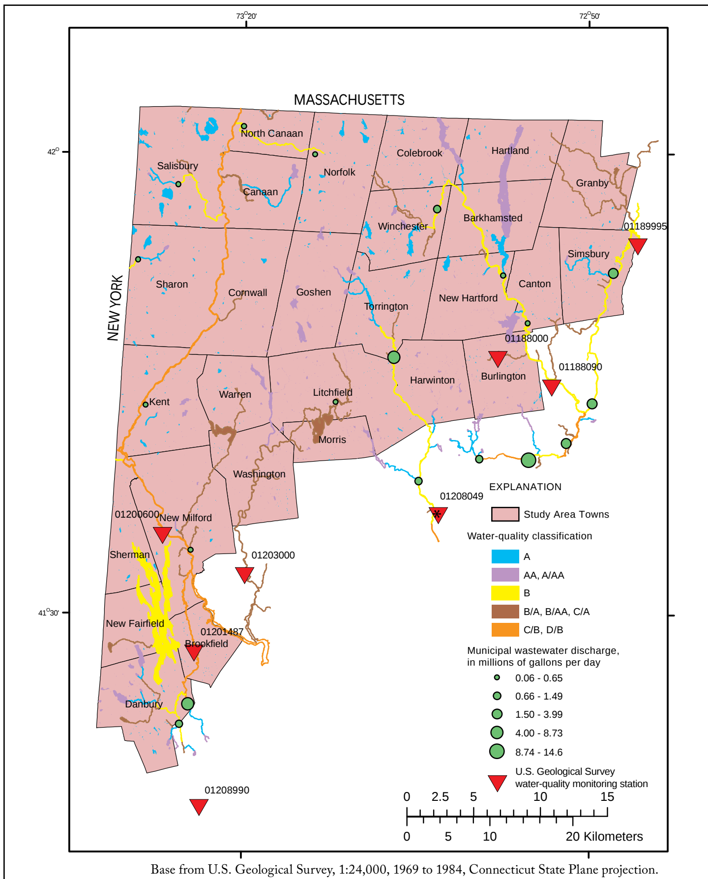
Figure CT-25. Water quality classification, municipal wastewater discharges, and U.S. Geological Survey long-term monitoring stations in the Connecticut Highlands study area. Class A indicates potential drinking water supply, Class AA indicates existing or proposed drinking water supply, Class B (non-drinking water supply) indicates other uses such as agricultural and industrial supply; and Class C indicates unacceptable quality.
