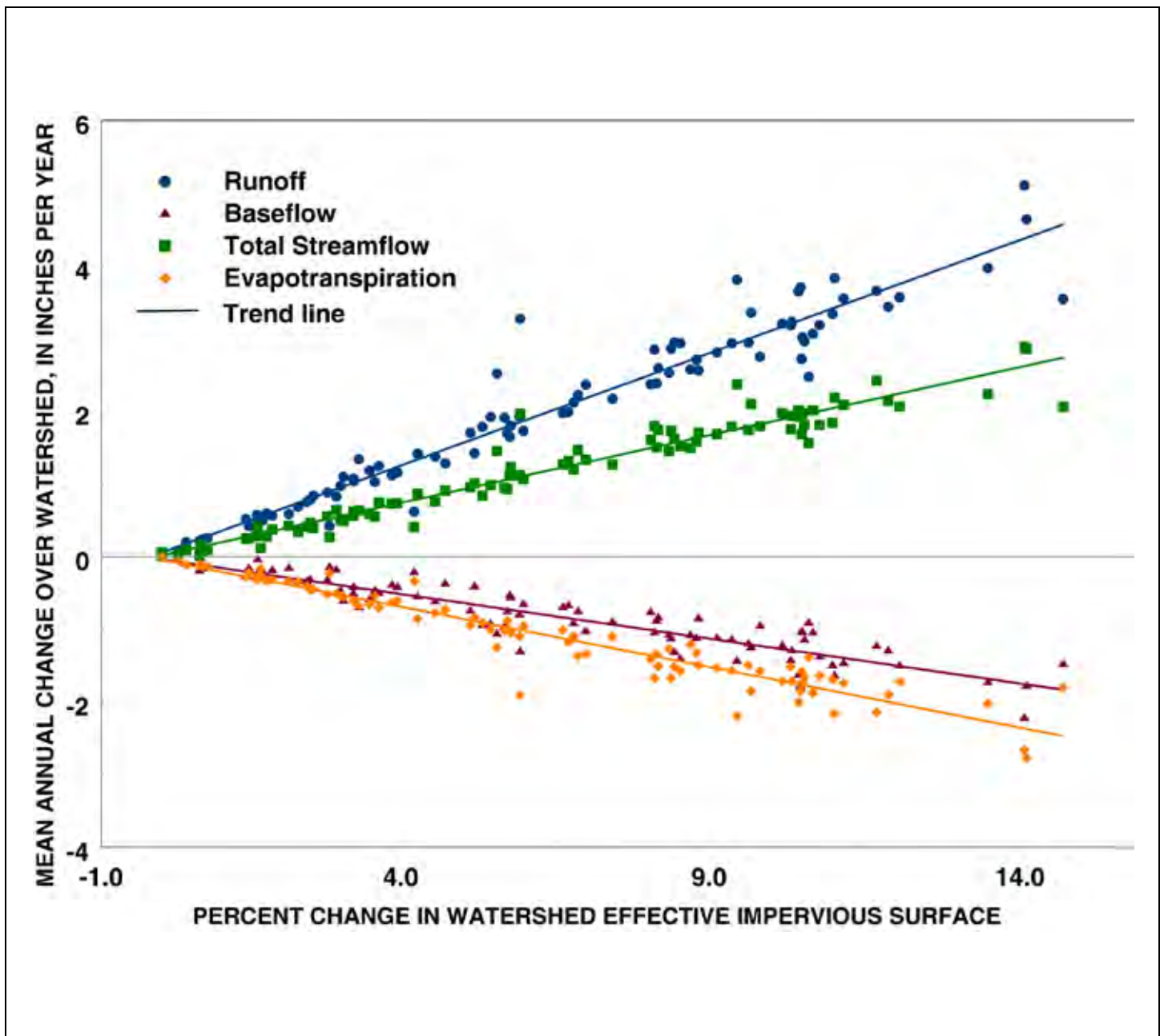
Figure PA-40. Effect of impervious surfaces on streamflow. Changes in streamflow characteristics and evapotranspiration are directly related to increasing impervious surface area, as shown here for 95 14-digit Hydrologic Unit Code subwatersheds in the Pennsylvania Highlands.
