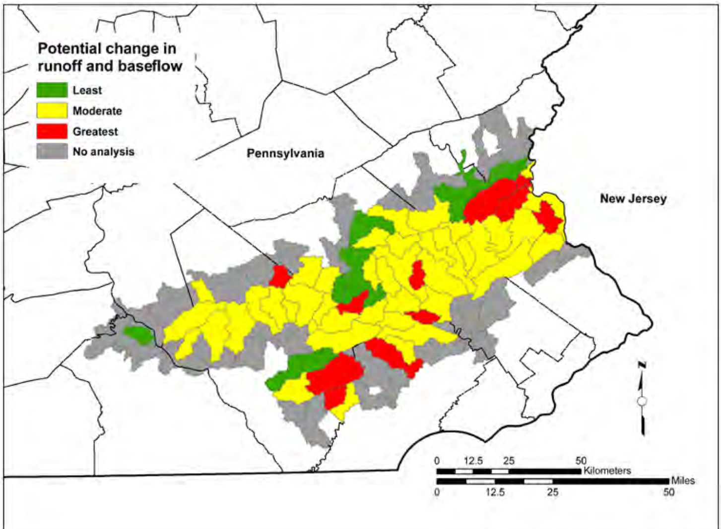
Figure PA-41. Predicted changes in streamflow. Predicted change in runoff and baseflow at the 14-digit Hydrologic Unit Code subwatershed scale in the Pennsylvania Highlands, based on the change between the simulated water budgets for 1986 – 2001 conditions and the low-constraint development scenario. The areas of moderate and greatest change in runoff and baseflow are directly related to the projected increase in impervious surface cover and water withdrawals.
