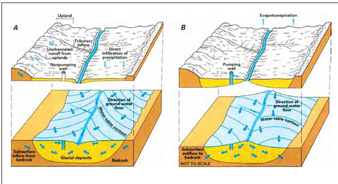
Figure CT-17. Recharge and flow in glacial aquifers. Ground water enters glacial aquifers in three ways: as runoff from the surface of surrounding bedrock, as underground flow from adjacent bedrock, and by infiltration of precipitation that falls directly over the aquifer. (A) When the water level in a glacial aquifer is above that in streams, ground water flows from aquifer to stream. (B) When the water level in a glacial aquifer drops below that in streams due to withdrawal from wells, drought, evapotranspiration, and seepage into adjacent bedrock, water flows from stream to aquifer (modified from Rosenshein 1988, p. 186).
