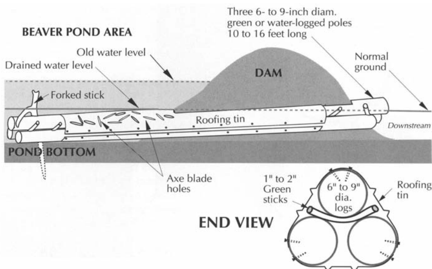
Figure 9. Three-log drain used to help control water levels in beaver ponds. Reprinted from Arner et al (1966).
