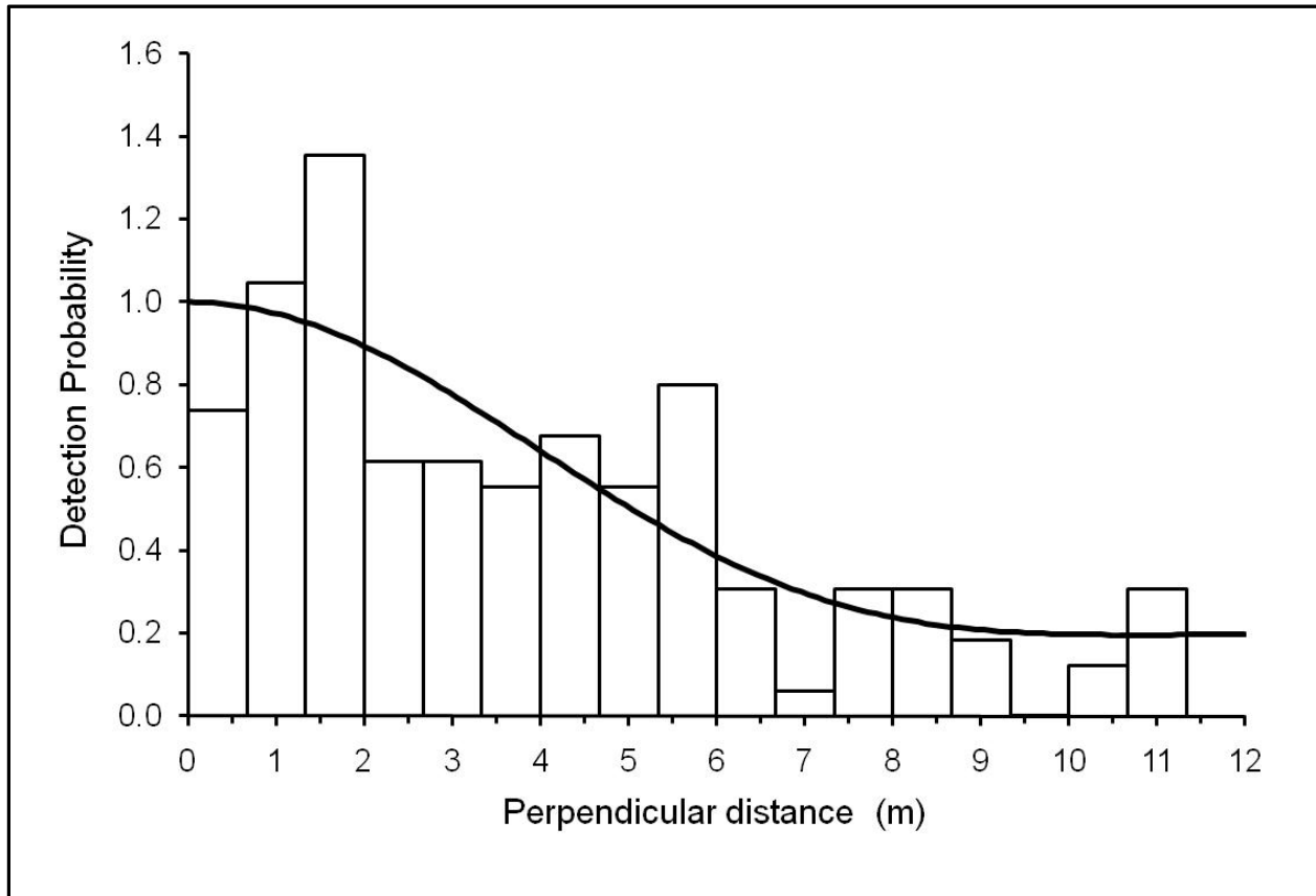
Figure 10. Observed detections (histogram) and the resulting detection function (smooth curve) for live tortoises with MCL \geq 180\text{mm} found by Kiva. Observations were truncated at 12m.
