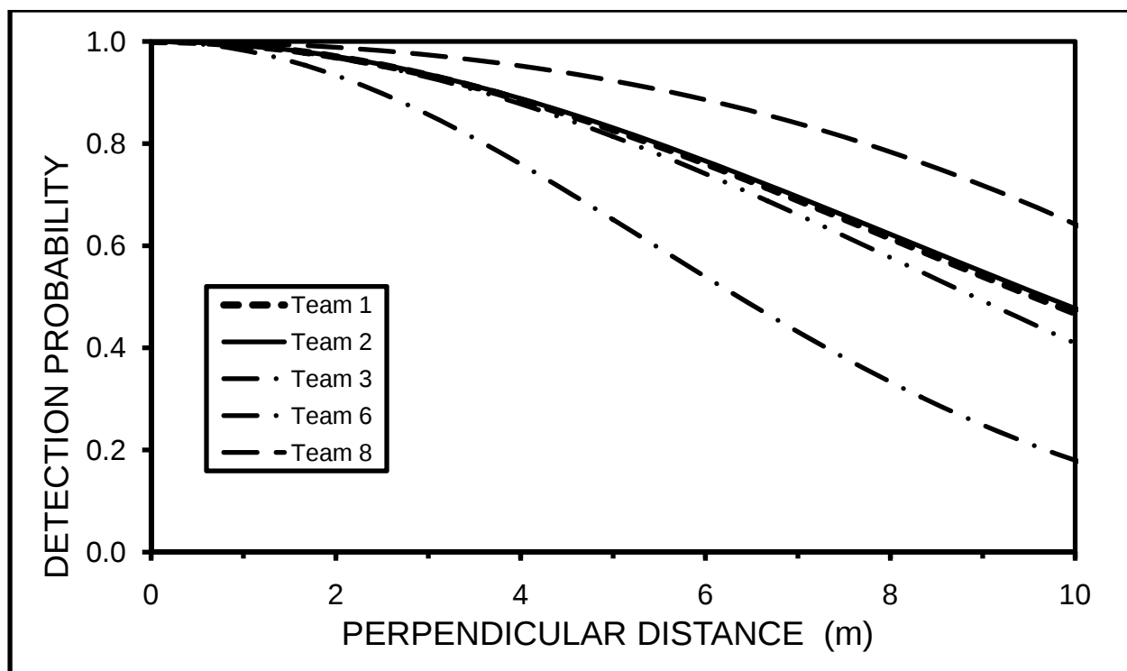
Figure 4. Detection curves for each of the 2007 trainee teams that returned after at least one year of monitoring experience. Curves are based on 16km trials.
