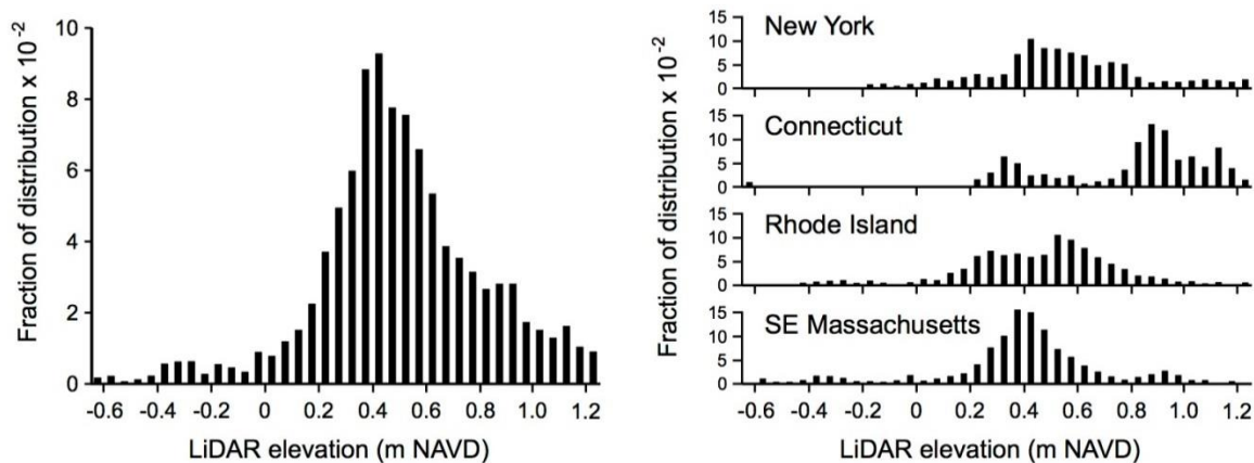
Distribution of salt marsh elevations for 38 Northeastern salt marshes
