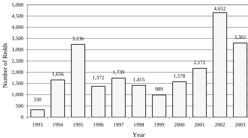
Figure 4. Yearly USFWS Chinook salmon redd counts, 1993 to 2003.
