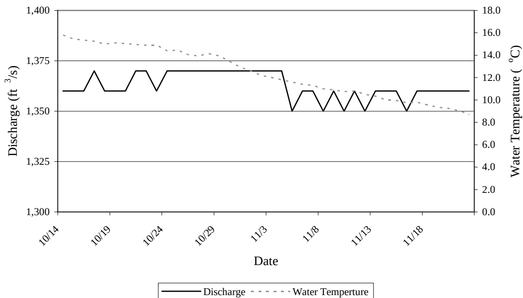
Figure 11. Water temperature (°C) at rkm 304.8 and discharge (ft 3 /s) from Iron Gate Dam (October 14 to November 22, 2003).
