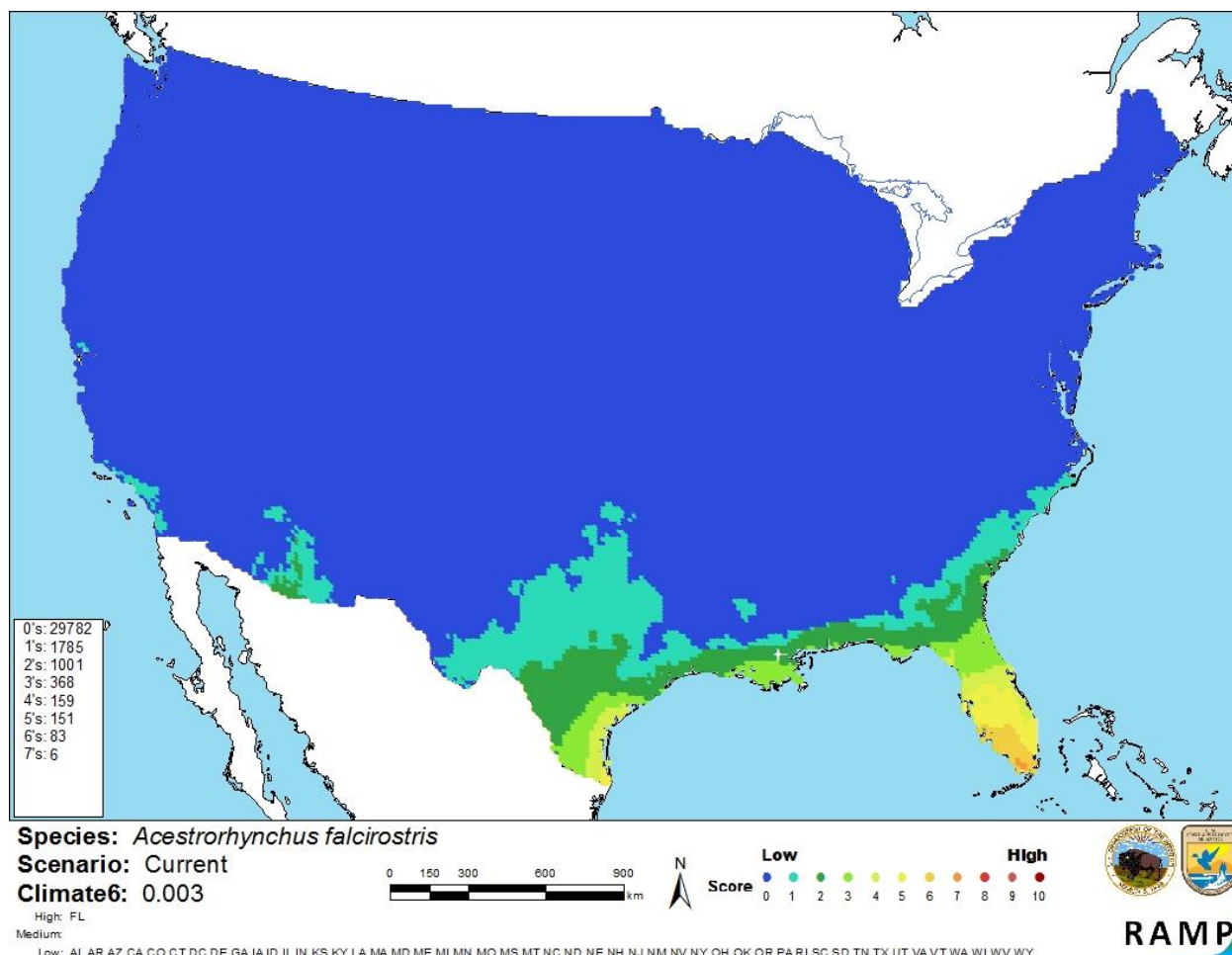
Figure 3. Map of RAMP (Sanders et al. 2014; 16 climate variables; Euclidean Distance) climate matches for Acestrorhynchus falcirostris in the contiguous United States based on source locations reported by GBIF Secretariat (2017). 0= Lowest match, 10=Highest match.
