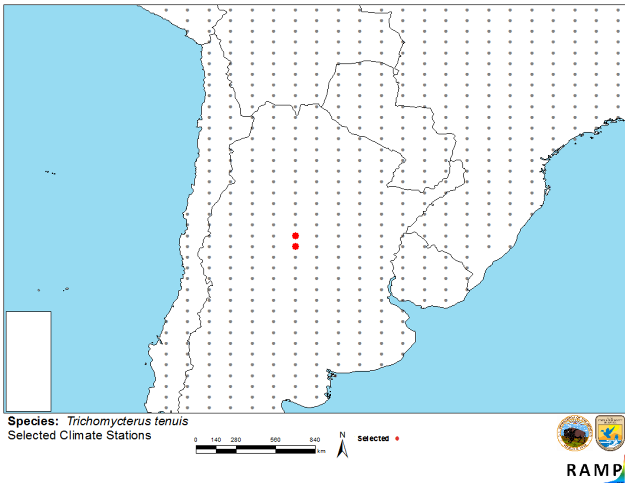
Figure 2. RAMP (Sanders et al. 2014) source map showing weather stations selected as source locations (red; north-central Argentina) and non-source locations (gray) for Trichomycterus tenuis climate matching. Source locations estimated from verbal description in Eschmeyer et al. (2016).
