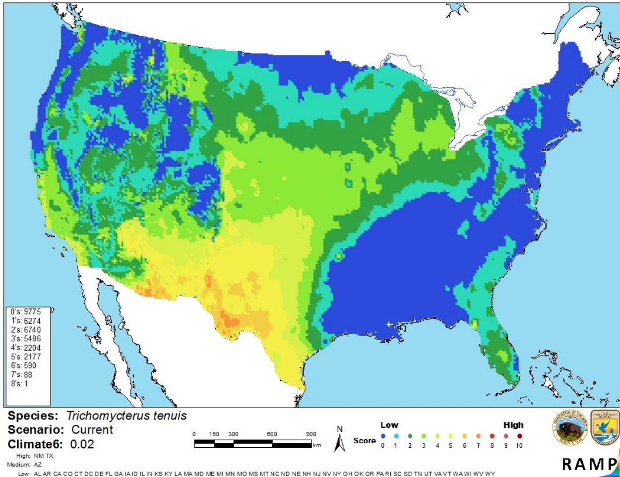
Figure 3. Map of RAMP (Sanders et al. 2014) climate matches for Trichomycterus tenuis in the contiguous United States based on source locations reported by Eschmeyer et al. (2016). 0= Lowest match, 10= Highest match. Counts of climate match scores are tabulated on the left.
