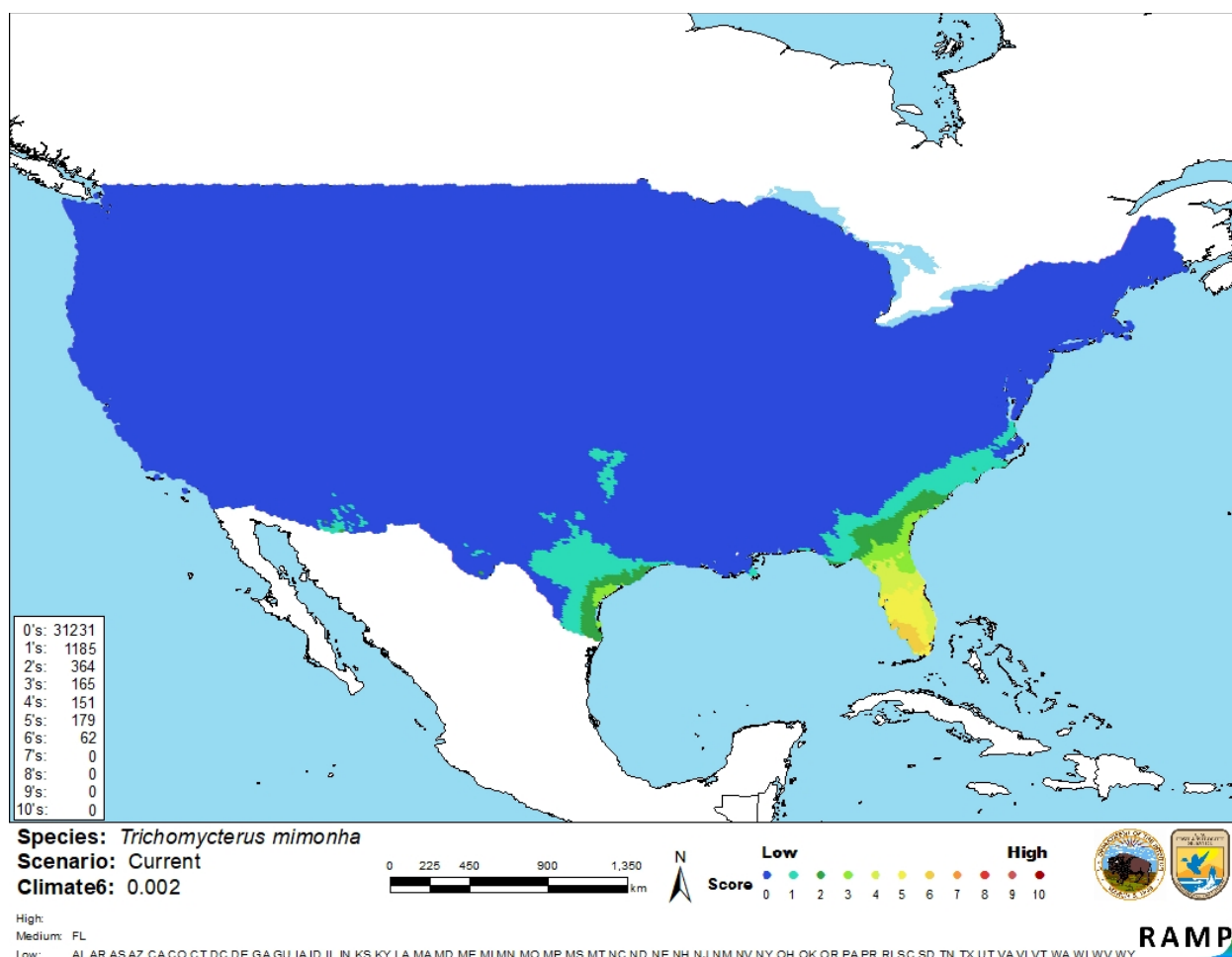
Figure 3. Map of RAMP (Sanders et al. 2018) climate matches for Trichomycterus mimonha in the contiguous United States based on source locations reported by GBIF Secretariat (2017). Counts of climate match scores are tabulated on the left. 0/Blue = Lowest match, 10/Red = Highest match.
