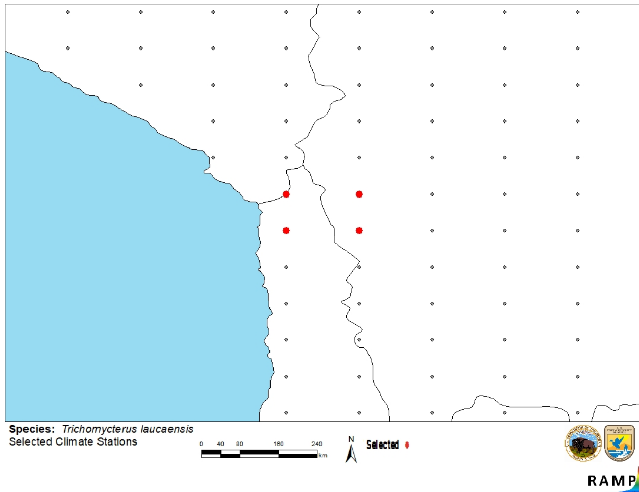
Figure 2. RAMP (Sanders et al. 2018) source map showing weather stations in South America selected as source locations (red; Chile, Bolivia) and non-source locations (gray) for Trichomycterus laucaensis climate matching. Source locations from GBIF Secretariat (2017). Selected source locations are within 100 km of one or more species occurrences and do not necessarily represent the locations of occurrences themselves.
