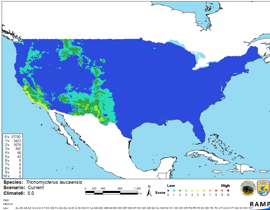
Figure 3. Map of RAMP (Sanders et al. 2018) climate matches for Trichomycterus laucaensis in the contiguous United States based on source locations reported by GBIF Secretariat (2017). Counts of climate match scores are tabulated on the left. 0/Blue = Lowest match, 10/Red = Highest match.
