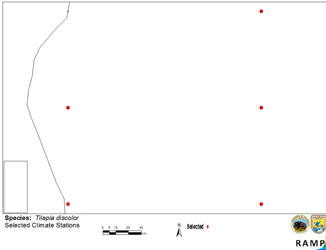
Figure 2. RAMP (Sanders et al. 2014) source map showing weather stations selected as source locations (red) and non-source locations (gray) for T. discolor climate matching. Source locations from GBIF (2015). Source locations are in Côte d'Ivoire and Ghana.
