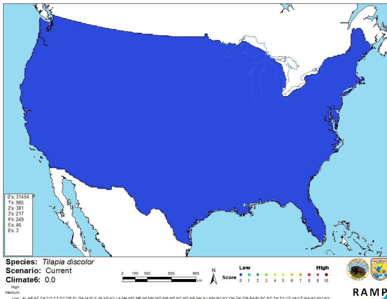
Figure 3. Map of RAMP (Sanders et al. 2014) climate matches for T. discolor in the continental United States based on source locations reported by GBIF (2015). 0= Lowest match, 10=Highest match. Counts of climate match scores are tabulated on the left.
