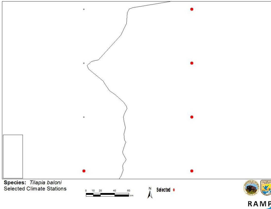
Figure 2. RAMP (Sanders et al. 2014) source map showing weather stations selected as source locations (red) and non-source locations (gray) for T. baloni climate matching. Source locations from GBIF (2015). Source locations are all in Zambia.
