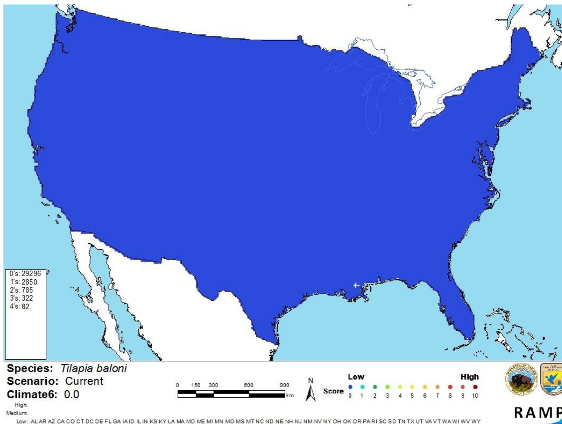
Figure 3. Map of RAMP (Sanders et al. 2014) climate matches for T. baloni in the continental United States based on source locations reported by GBIF (2015). 0= Lowest match, 10=Highest match. Counts of climate match scores are tabulated on the left.
