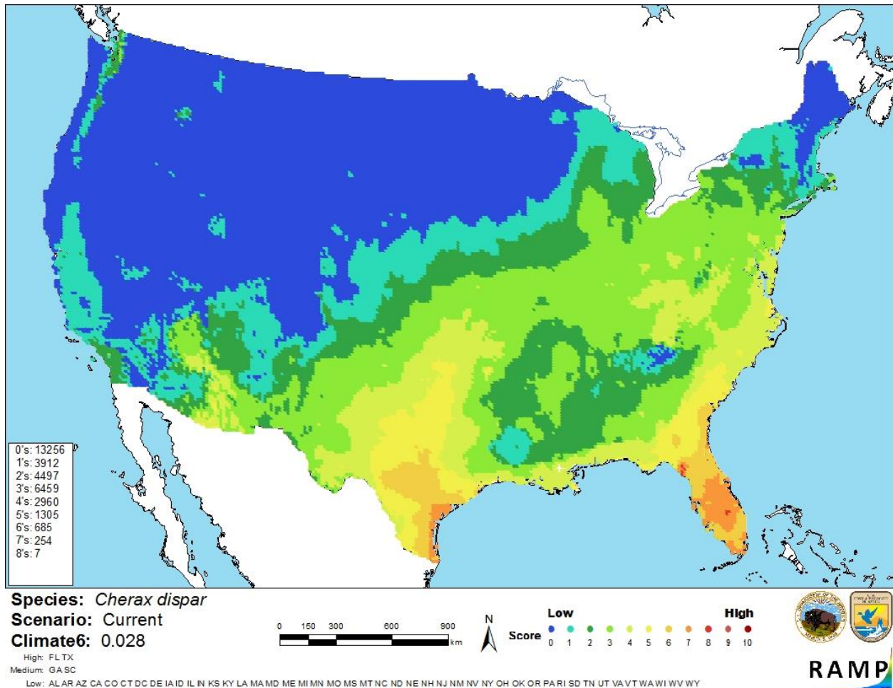
Figure 3. Map of RAMP (Sanders et al. 2014) climate matches for Cherax dispar in the contiguous United States based on source locations reported by GBIF Secretariat (2017). 0=Lowest match, 10=Highest match.
