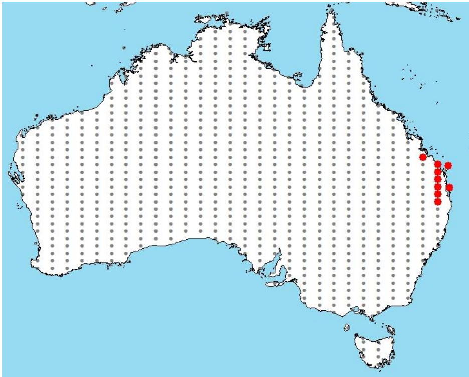
Figure 2. RAMP (Sanders et al. 2014) source map showing weather stations in Australia selected as source locations (red) and non-source locations (gray) for Cherax dispar climate matching. Source locations from GBIF Secretariat (2017).
