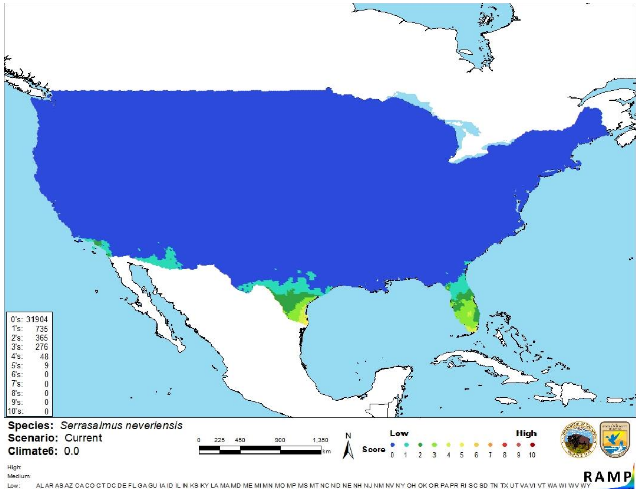
Figure 3. Map of RAMP (Sanders et al. 2018) climate matches for Serrasalmus neveriensis in the contiguous United States based on source locations reported by Fricke et al. (2020). Counts of climate match scores are tabulated on the left. 0/Blue = Lowest match, 10/Red = Highest match.
