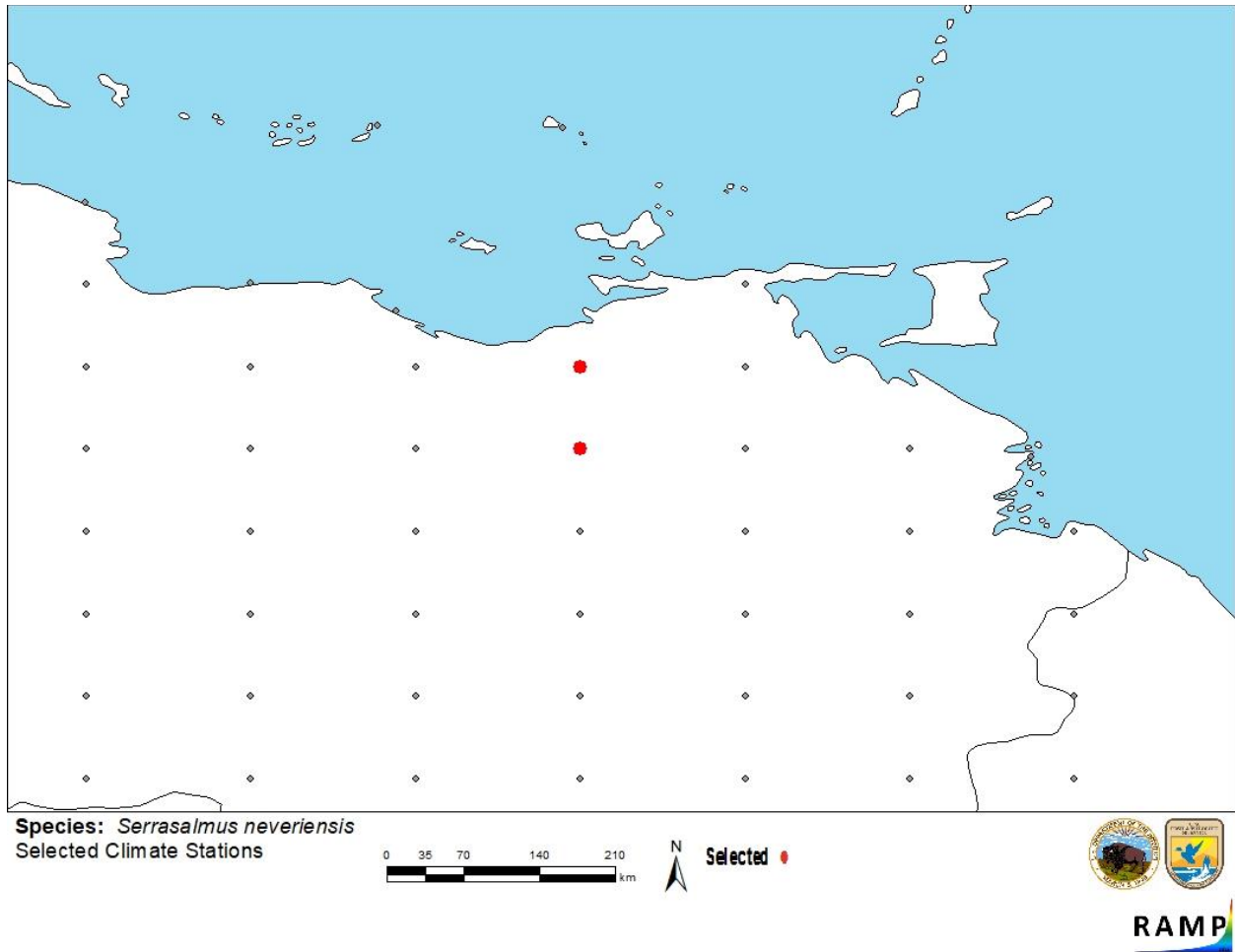
Figure 2. RAMP (Sanders et al. 2018) source map showing weather stations in northeastern Venezuela selected as source locations (red; Venezuela) and non-source locations (gray) for Serrasalmus neveriensis climate matching. Source locations estimated from verbal description of type locality in Fricke et al. (2020). Selected source locations are within 100 km of one or more species occurrences, and do not necessarily represent the locations of occurrences themselves.
