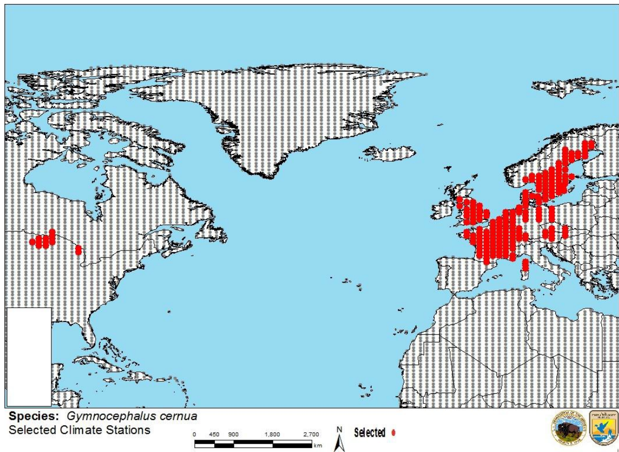
Figure 3. RAMP (Sanders et al. 2014) source map showing weather stations selected as source locations (red) and non-source locations (blue) for Gymnocephalus cernua climate matching. Source locations from GBIF (2015).
