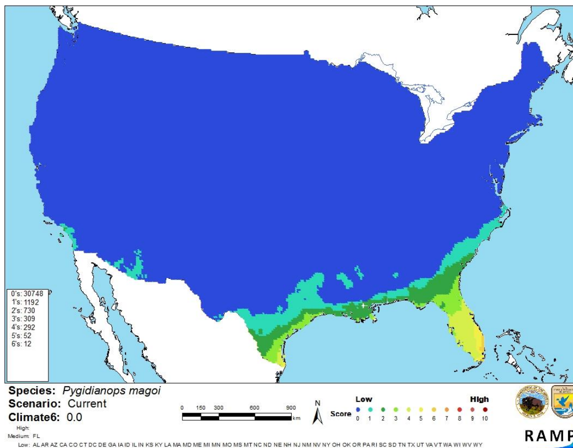
Figure 3. Map of RAMP (Sanders et al. 2014) climate matches for Pygidianops magoi in the contiguous United States based on source locations reported by Schaefer et al. (2005). 0= Lowest match, 10=Highest match. Counts of climate match scores are tabulated on the left.
