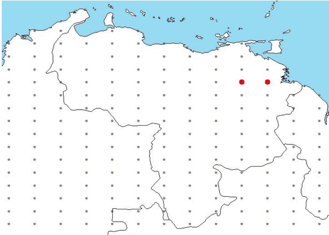
Figure 2. RAMP (Sanders et al. 2014) source map showing weather stations selected as source locations (red; Venezuela) and non-source locations (gray) for Pygidianops magoi climate matching. Source locations from Schaefer et al. (2005).
