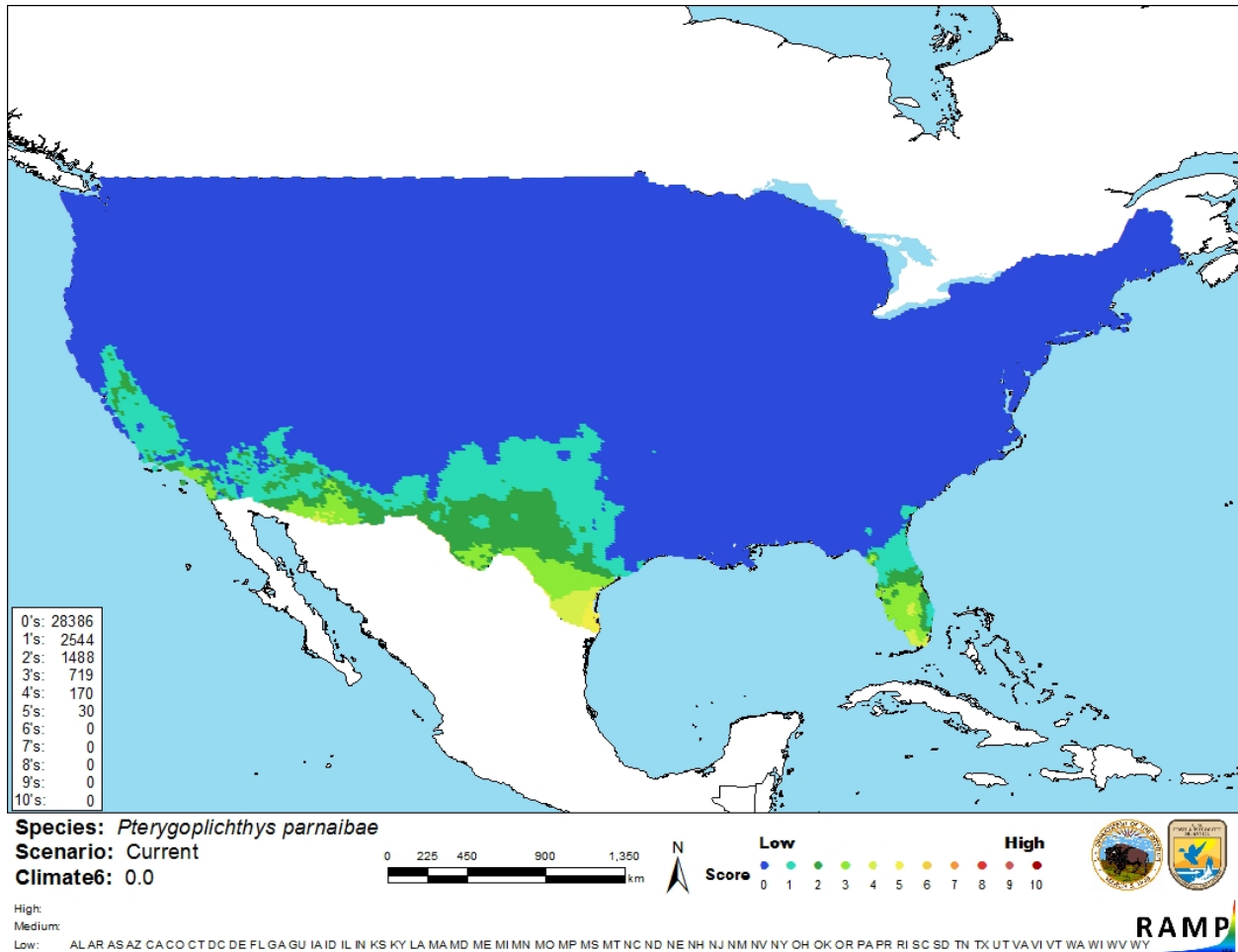
Figure 3. Map of RAMP (Sanders et al. 2018) climate matches for Pterygoplichthys parnaibae in the contiguous United States based on source locations reported from GBIF Secretariat (2018). Counts of climate match scores are tabulated on the left. 0/Blue = Lowest match, 10/Red = Highest match.
