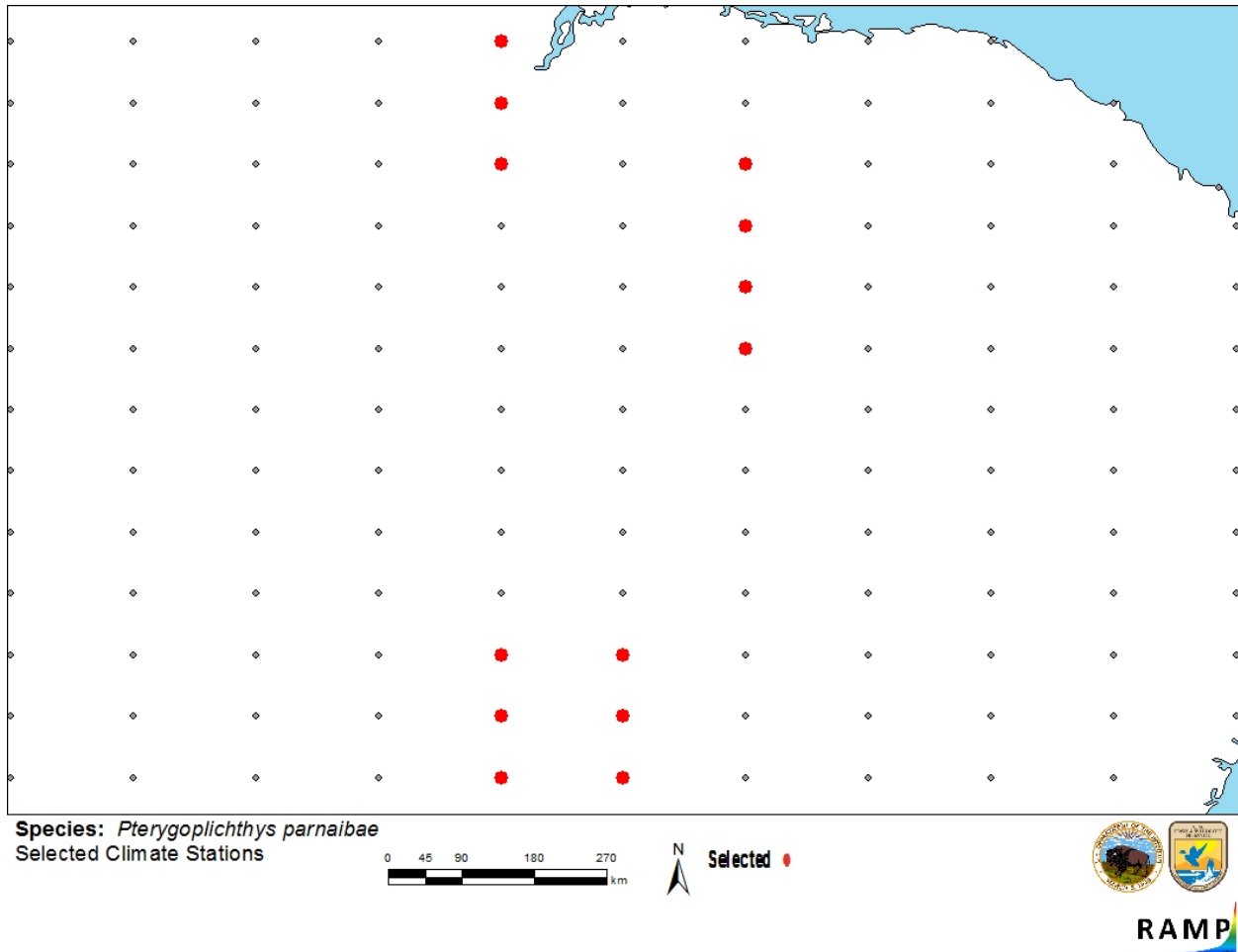
Figure 2. RAMP (Sanders et al. 2018) source map showing weather stations in northern South America selected as source locations (red; Brazil) and non-source locations (gray) for Pterygoplichthys parnaibae climate matching. Source locations from GBIF Secretariat (2018). Selected source locations are within 100 km of one or more species occurrences, and do not necessarily represent the locations of occurrences themselves.
