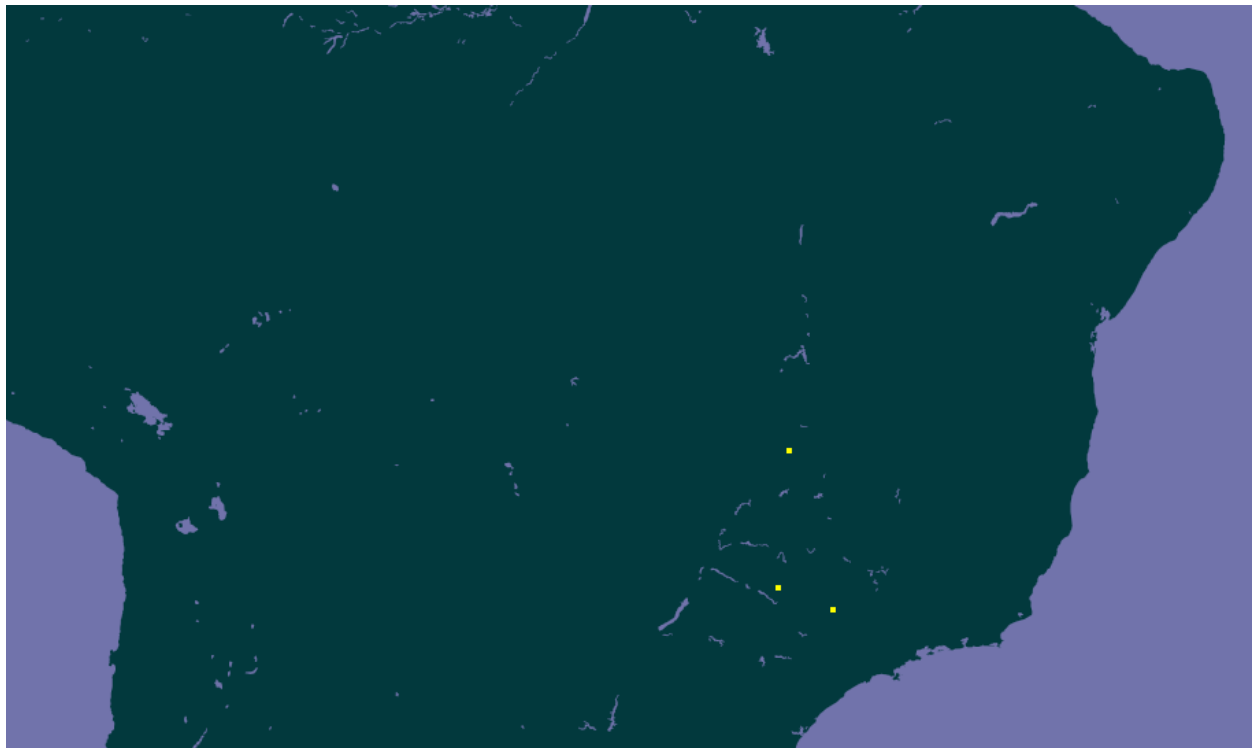
Figure 1. Reported distribution of Parastegophilus paulensis in Brazil. Map from GBIF (2016).
