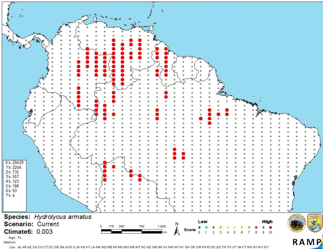
Figure 2. RAMP (Sanders et al. 2014) source map showing weather stations selected as source locations (red; Bolivia, Brazil, Colombia, Guyana, Venezuela) and non-source locations (gray) for Hydrolycus armatus climate matching. Source locations from GBIF Secretariat (2017).
