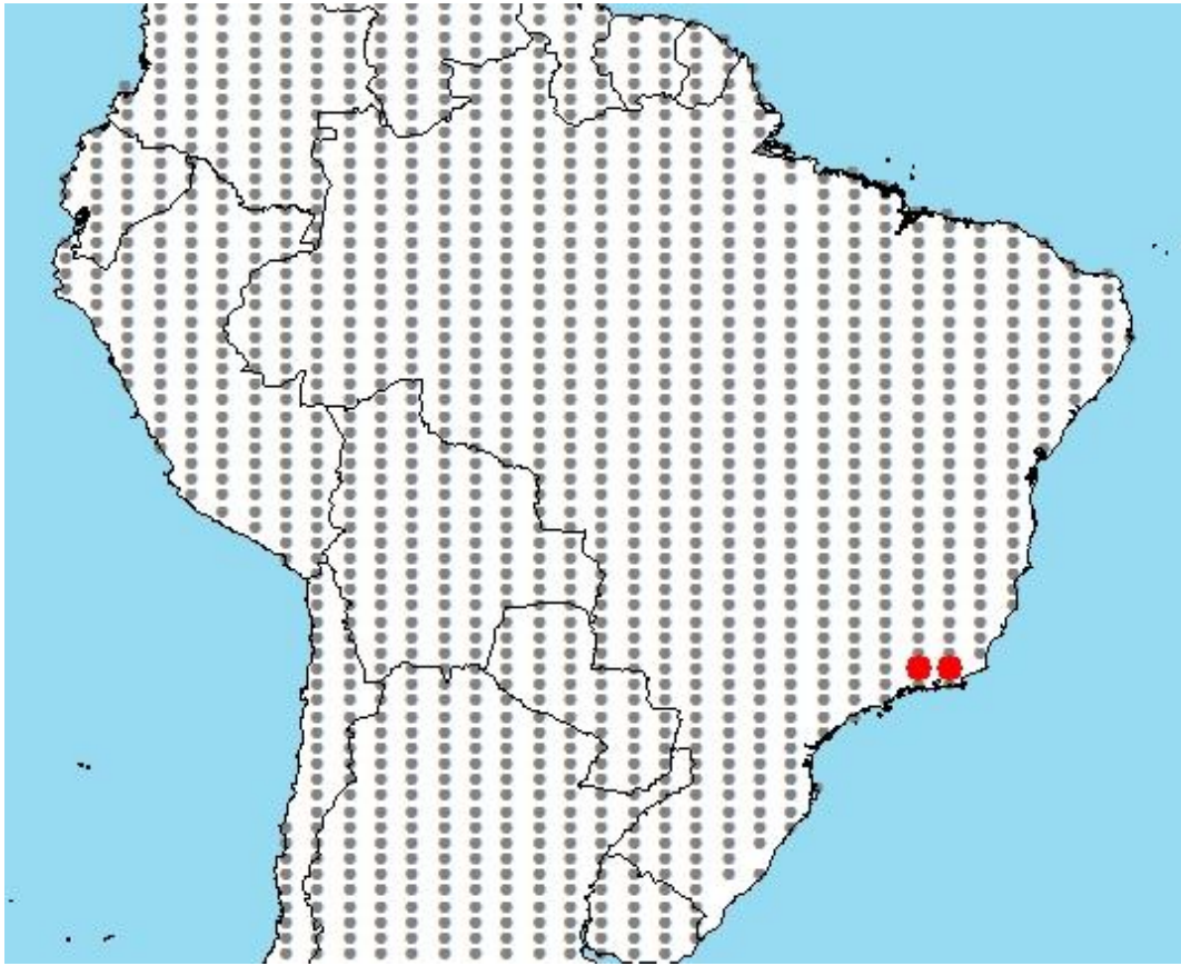
Figure 1. RAMP (Sanders et al. 2014) source map of South America showing weather stations selected as source locations (red; in southeastern Brazil) and non-source locations (gray) for Listrura nematopteryx climate matching. Source locations from GBIF (2016).
