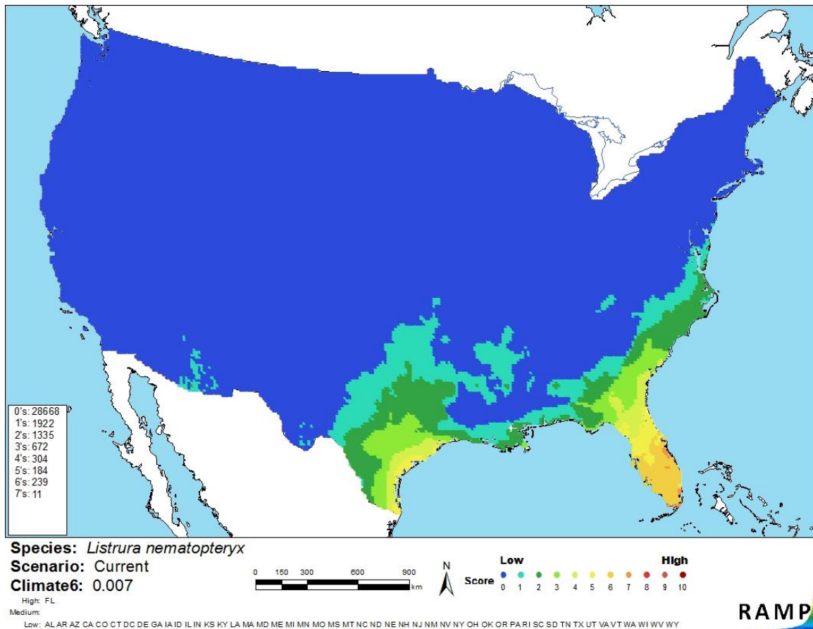
Figure 2. Map of RAMP (Sanders et al. 2014) climate matches for Listrura nematopteryx in the contiguous United States based on source locations reported by GBIF (2016). 0=Lowest match, 10=Highest match. Counts of climate match scores are tabulated on the left.
