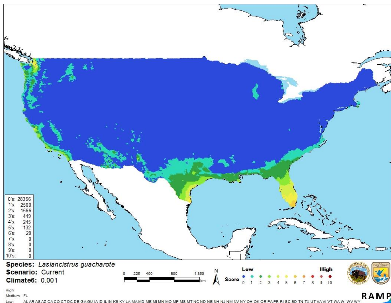
Figure 3. Map of RAMP (Sanders et al. 2018) climate matches for Lasiancistrus guacharote in the contiguous United States based on source locations reported from GBIF Secretariat (2019). Counts of climate match scores are tabulated on the left. 0 = Lowest match, 10 = Highest match.
