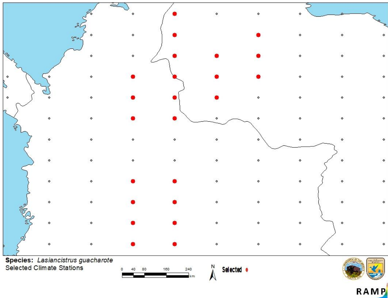
Figure 2. RAMP (Sanders et al. 2018) source map showing weather stations in South America selected as source locations (red; Colombia, Venezuela) and non-source locations (gray) for Lasiancistrus guacharote climate matching. Source locations from GBIF Secretariat (2019).
