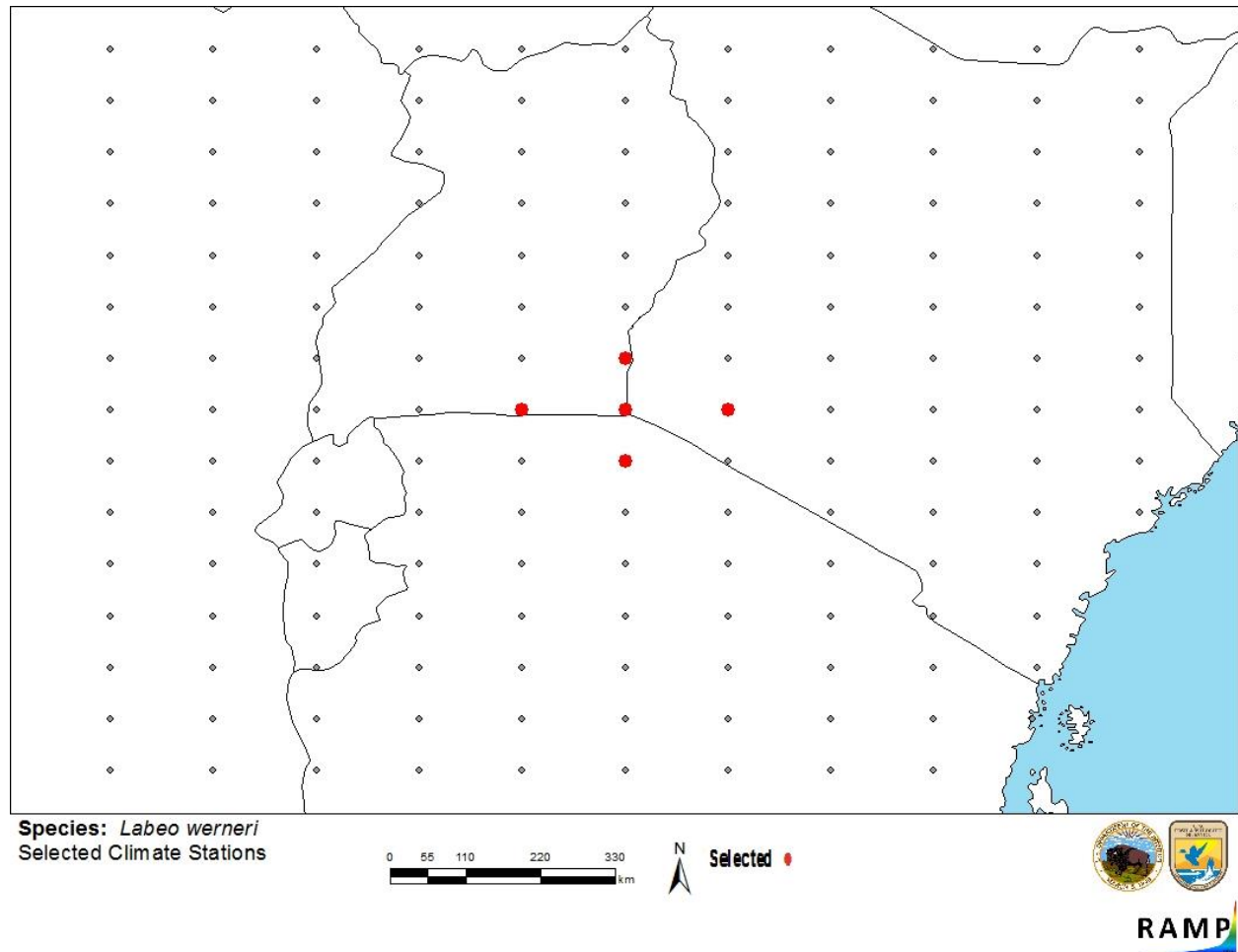
Figure 2. RAMP (Sanders et al. 2018) source map of east-central Africa showing weather stations selected as source locations (red; Lake Victoria in Kenya, Tanzania, and Uganda) and non-source locations (gray) for Labeo weneri climate matching. Source locations estimated from verbal description in Froese and Pauly (2018); no georeferenced occurrences available from GBIF Secretariat (2017).
