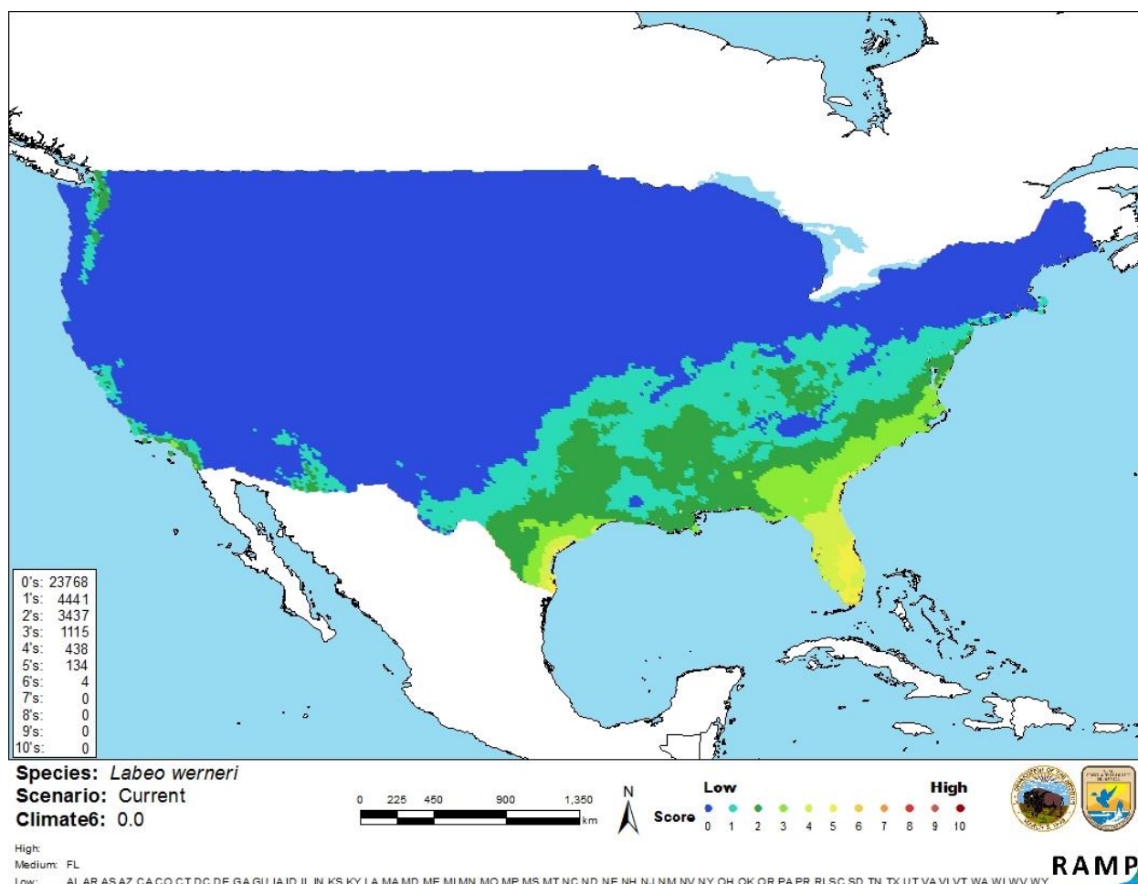
Figure 3. Map of RAMP (Sanders et al. 2018) climate matches for Labeo weneri in the contiguous United States based on source locations reported by Froese and Pauly (2018). 0=Lowest match, 10=Highest match.
