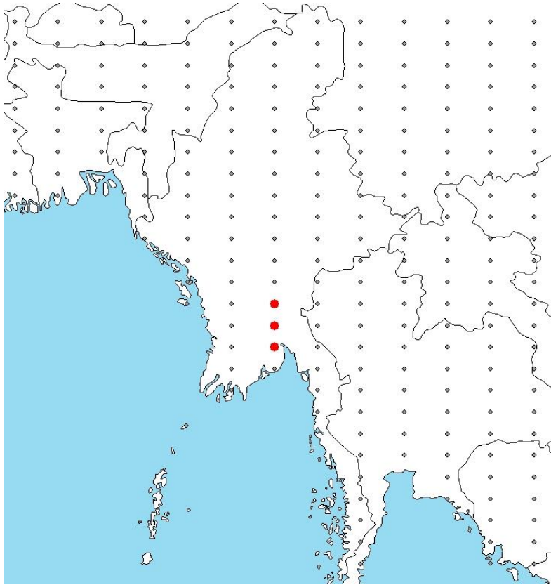
Figure 2. RAMP (Sanders et al. 2018) source map showing weather stations selected as source locations (red; Myanmar) and non-source locations (gray) for L. stolizkae climate matching. Source locations from GBIF Secretariat (2017).
