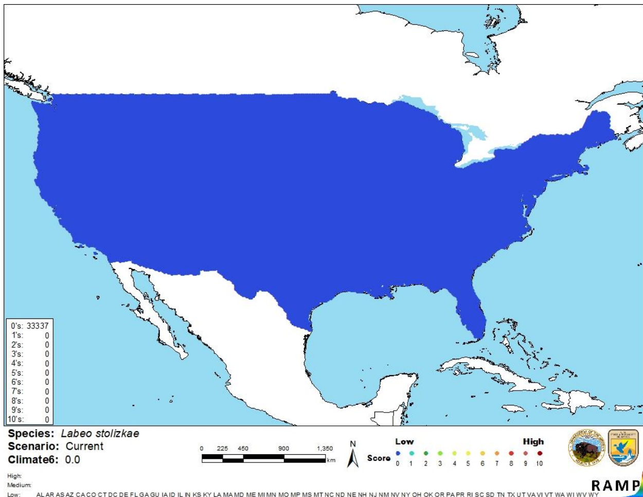
Figure 3. Map of RAMP (Sanders et al. 2018) climate matches for L. stolizkae in the contiguous United States based on source locations reported by GBIF Secretariat (2017). 0=Lowest match, 10=Highest match.
