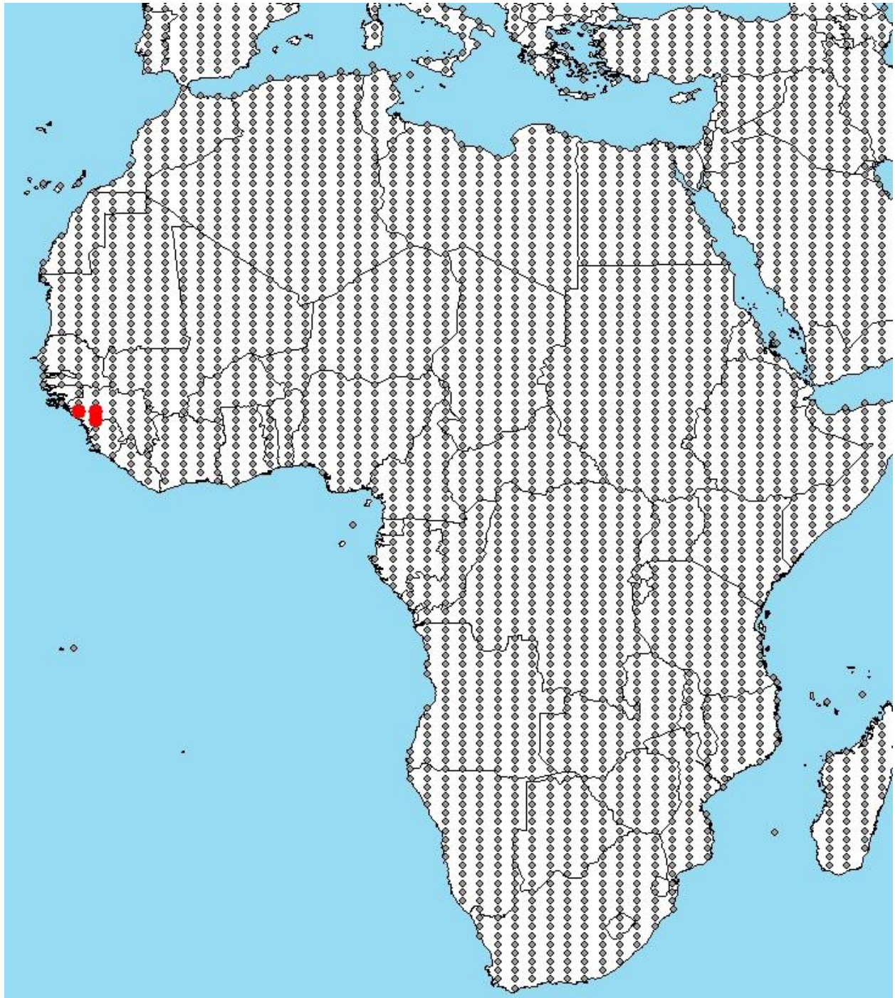
Figure 2. RAMP (Sanders et al. 2018) source map showing weather stations in West Africa selected as source locations (red; Guinea) and non-source locations (gray) for L. rouaneti climate matching. Source locations from GBIF Secretariat (2017).
