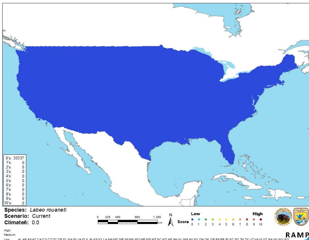
Figure 3. Map of RAMP (Sanders et al. 2018) climate matches for L. rouaneti in the contiguous United States based on source locations reported by GBIF Secretariat (2017). 0=Lowest match, 10=Highest match. Counts of climate match scores are tabulated on the left.
