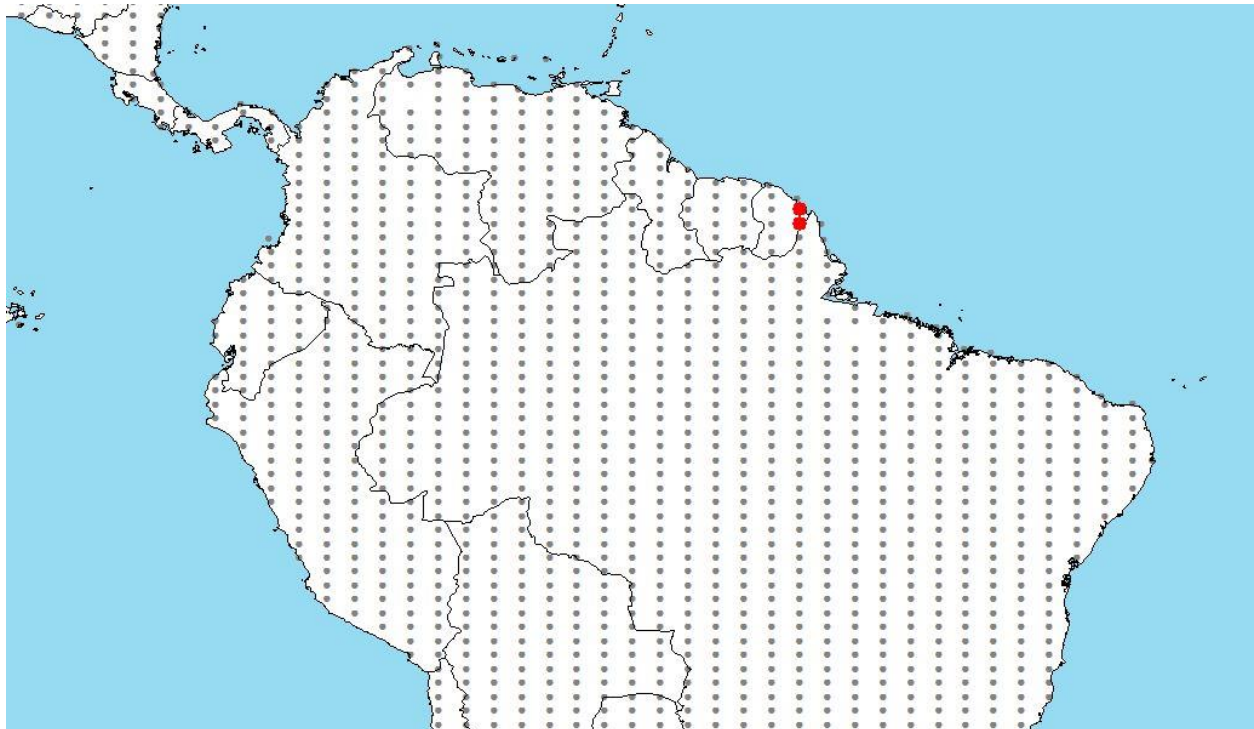
Figure 2. RAMP (Sanders et al. 2014) source map showing weather stations selected as source locations (red) and non-source locations (blue) for Ituglanis nebulosus climate matching. Source locations from GBIF (2016).
