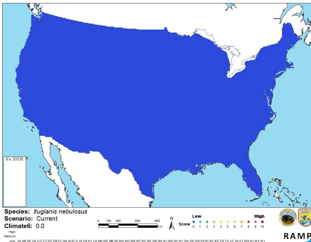
Figure 3. Map of RAMP (Sanders et al. 2014) climate matches for Ituglanis nebulosus in the contiguous United States based on source locations reported by GBIF (2016). 0= Lowest match, 10=Highest match. Counts of climate match scores are tabulated on the left.
