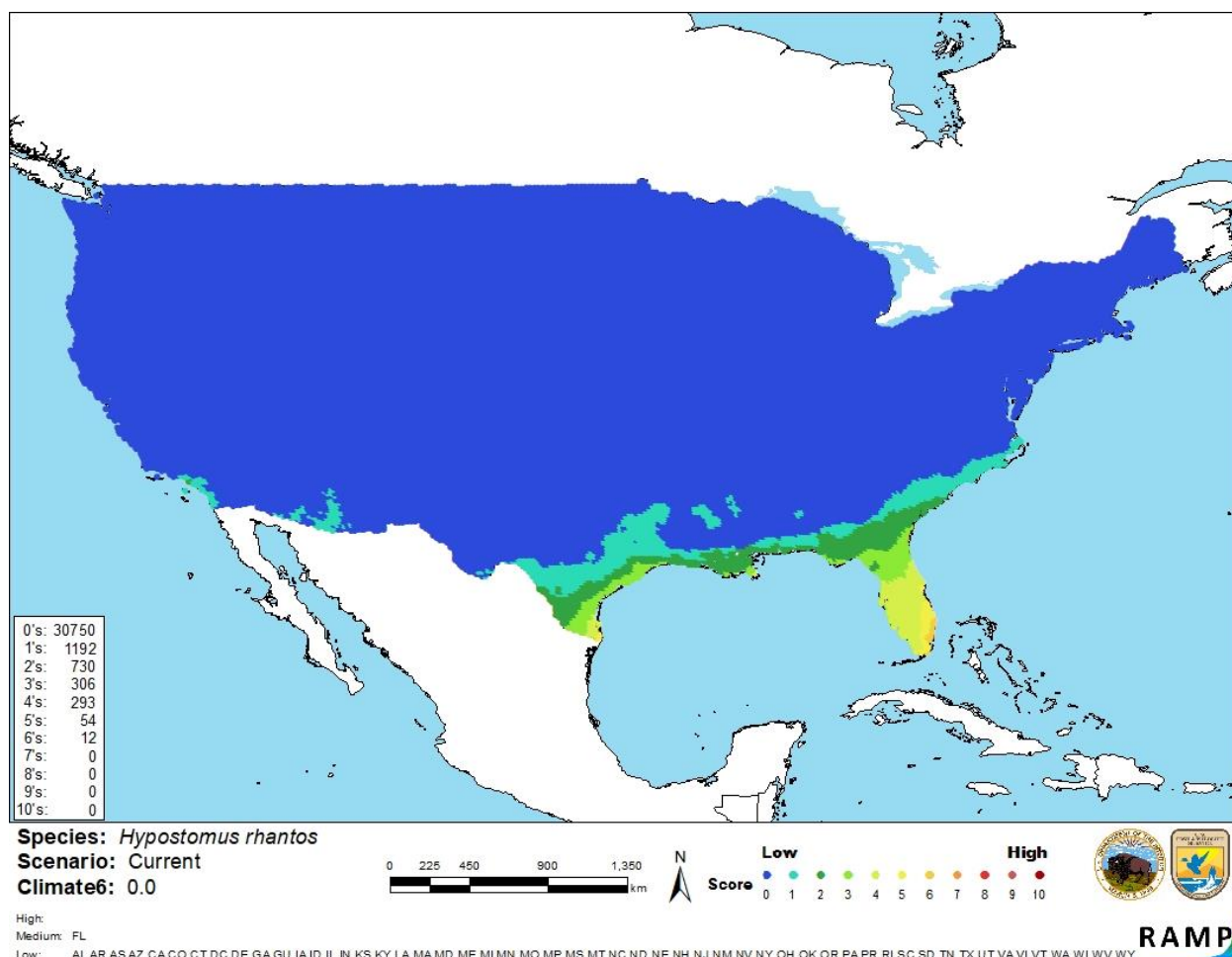
Figure 3. Map of RAMP (Sanders et al. 2018) climate matches for H. rhantos in the contiguous United States based on source locations reported by GBIF Secretariat (2017). 0= Lowest match, 10= Highest match.
