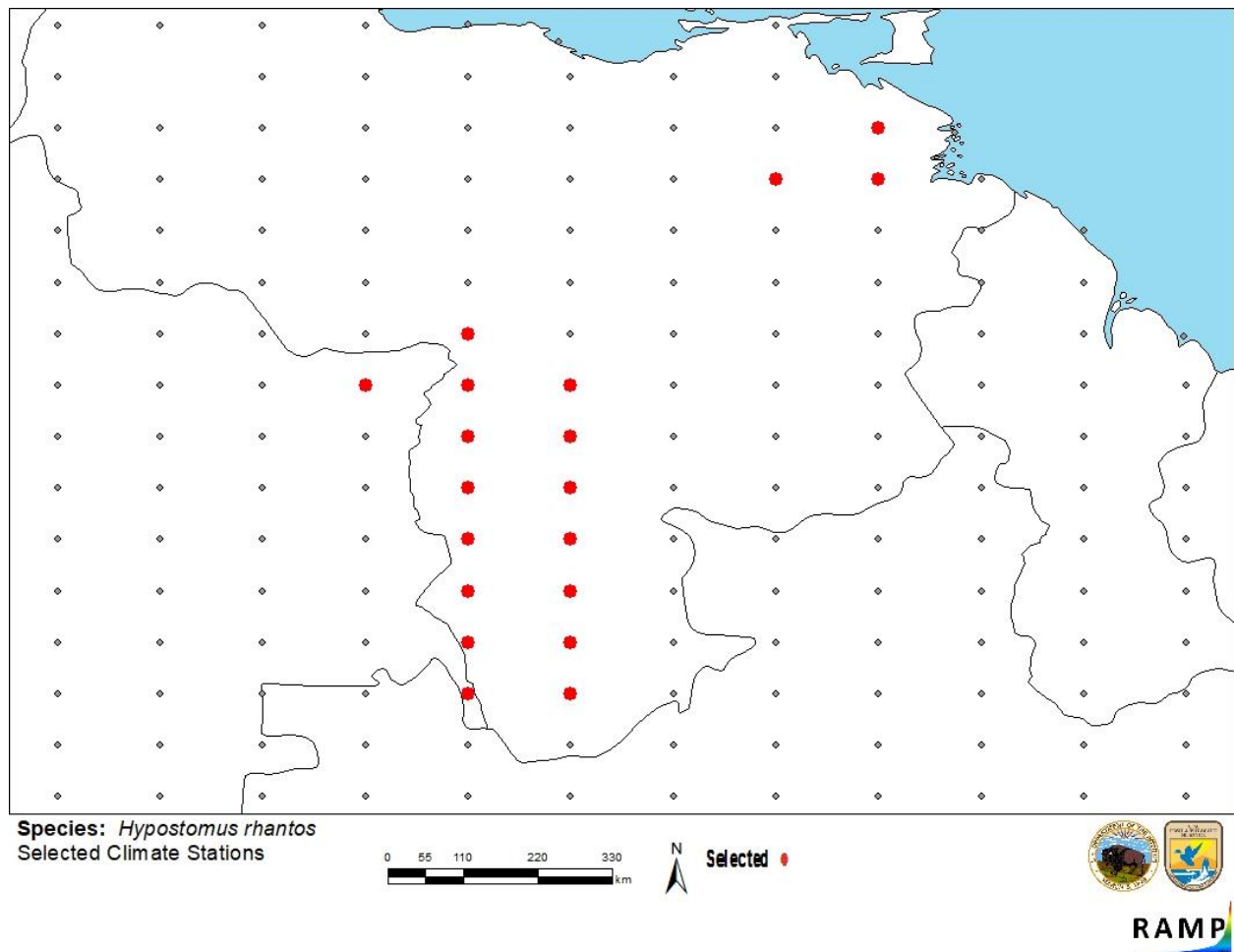
Figure 2. RAMP (Sanders et al. 2018) source map showing weather stations selected as source locations (red; Venezuela, Colombia) and non-source locations (gray) for H. rhanthos climate matching. Source locations from GBIF Secretariat (2017).
