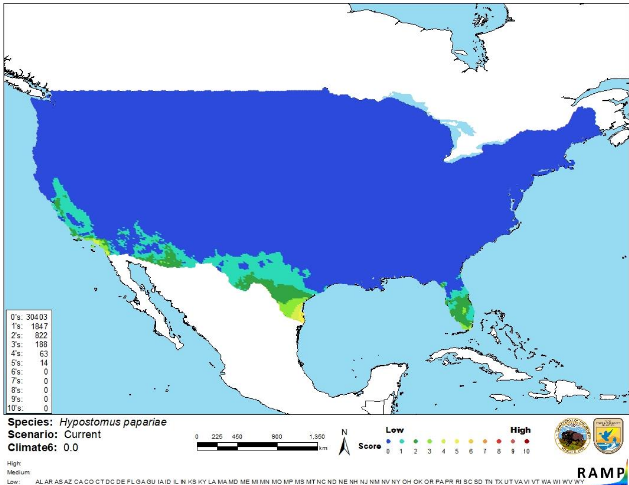
Figure 3. Map of RAMP (Sanders et al. 2018) climate matches for H. papariae in the contiguous United States based on source locations reported by Froese and Pauly (2018). 0= Lowest match, 10= Highest match.
