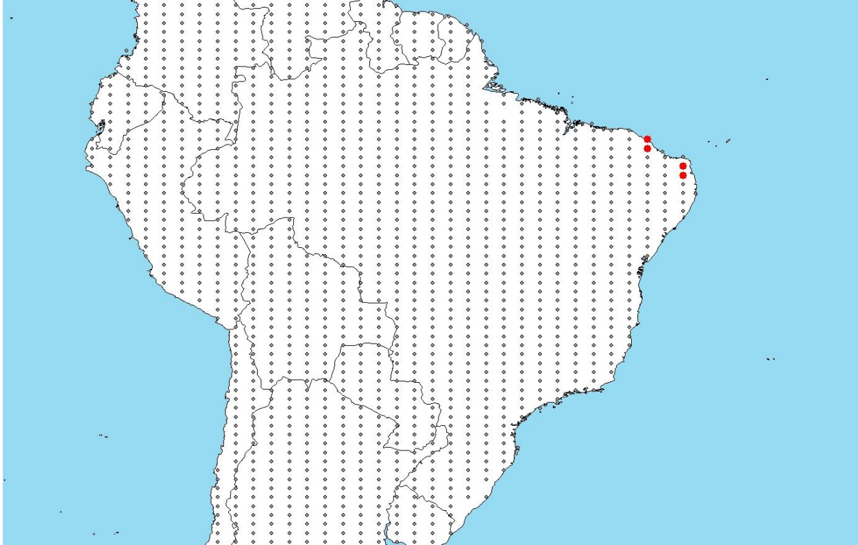
Figure 2. RAMP (Sanders et al. 2018) source map showing weather stations selected as source locations (red; Brazil) and non-source locations (gray) for H. papariae climate matching. Source locations from Froese and Pauly (2018).
