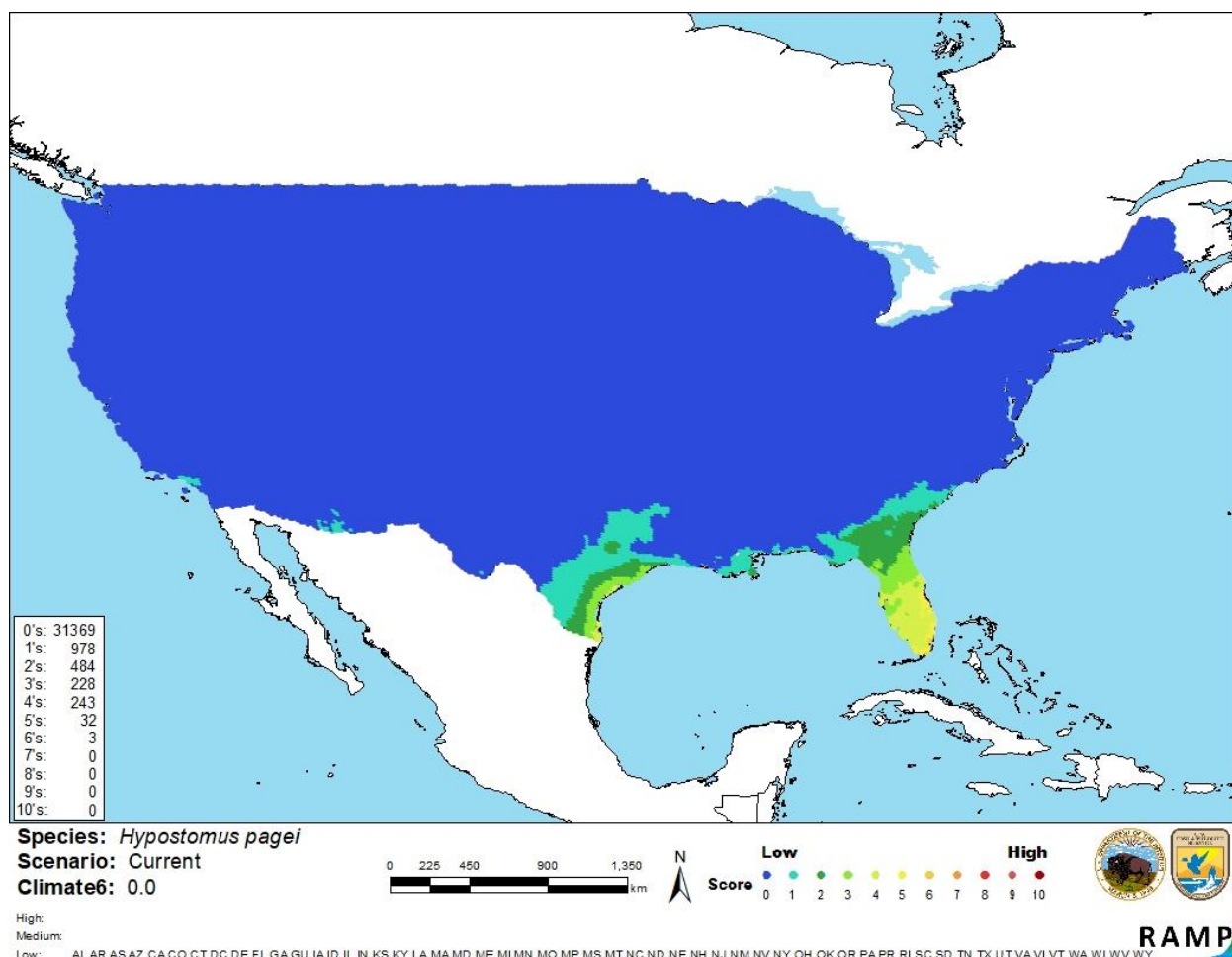
Figure 3. Map of RAMP (Sanders et al. 2018) climate matches for Hypostomus pagei in the contiguous United States based on source locations reported by GBIF Secretariat (2017). 0= Lowest match, 10= Highest match.
