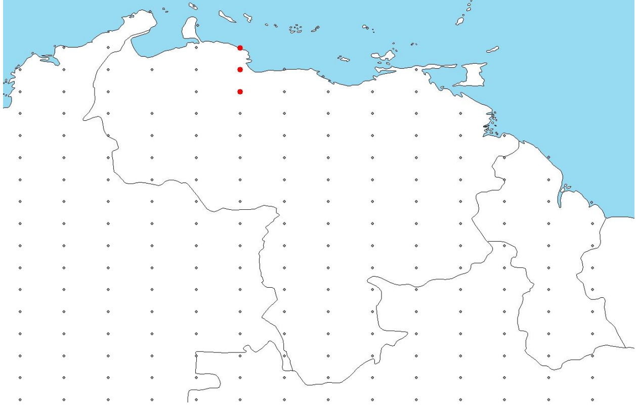
Figure 2. RAMP (Sanders et al. 2018) source map showing weather stations selected as source locations (red; Venezuela) and non-source locations (gray) for Hypostomus pagei climate matching. Source locations from GBIF Secretariat (2017).
