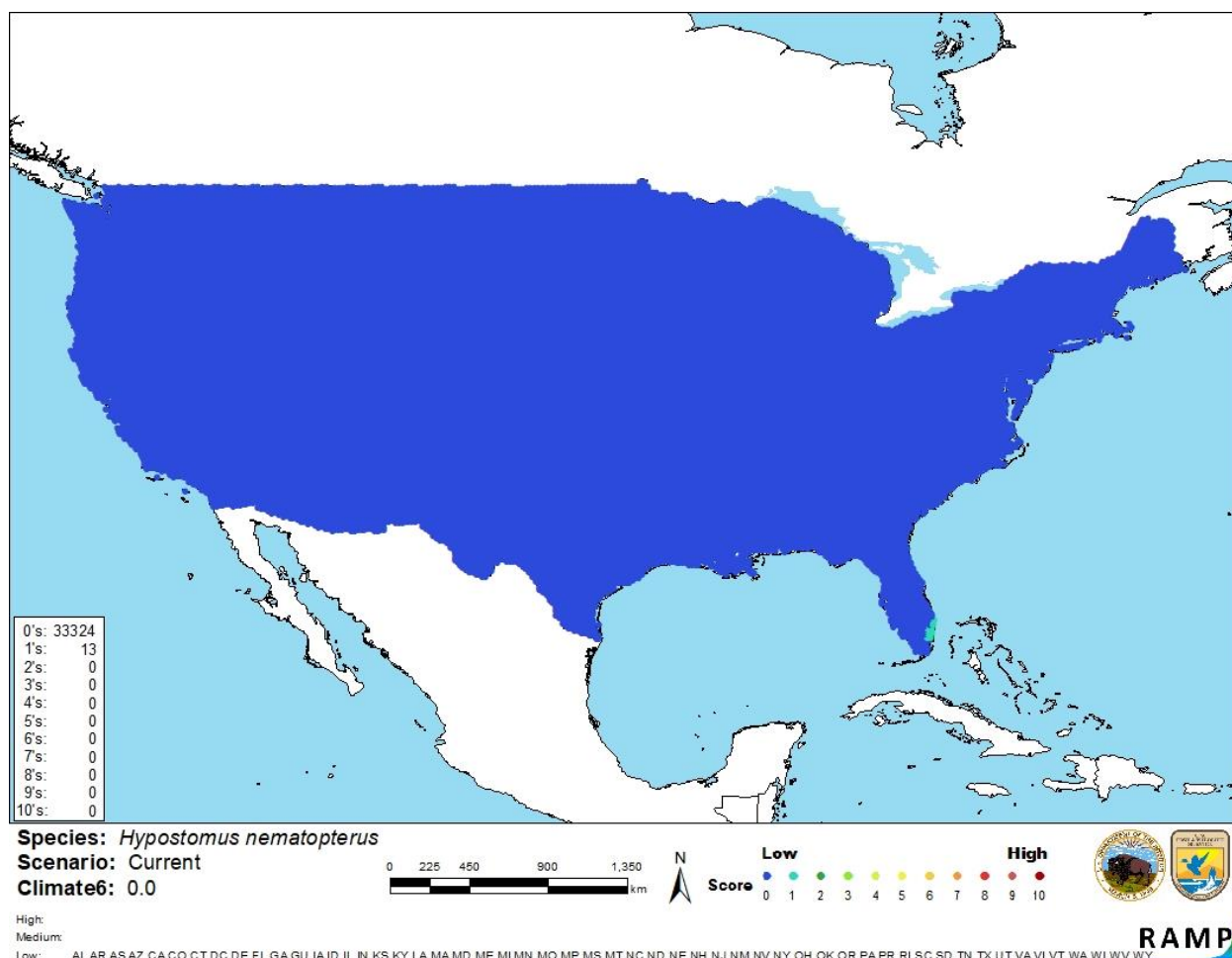
Figure 3. Map of RAMP (Sanders et al. 2018) climate matches for H. nematopterus in the contiguous United States based on source locations reported by Froese and Pauly (2018). 0= Lowest match, 10= Highest match.
