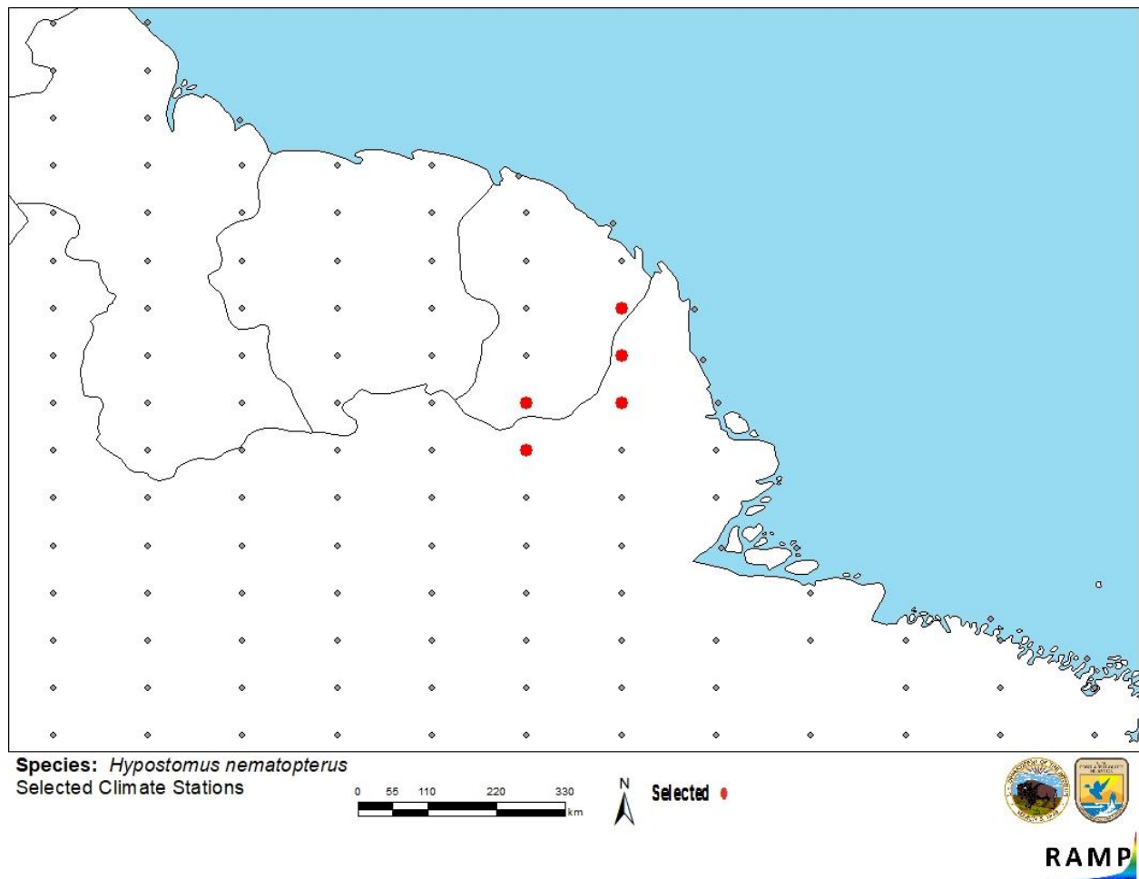
Figure 2. RAMP (Sanders et al. 2018) source map showing weather stations selected as source locations (red; French Guiana, Brazil) and non-source locations (gray) for H. nematopterus climate matching. Source locations from GBIF Secretariat (2017). Selected source locations are within 100 km of one or more species occurrences, and do not necessarily represent the locations of occurrences themselves.
