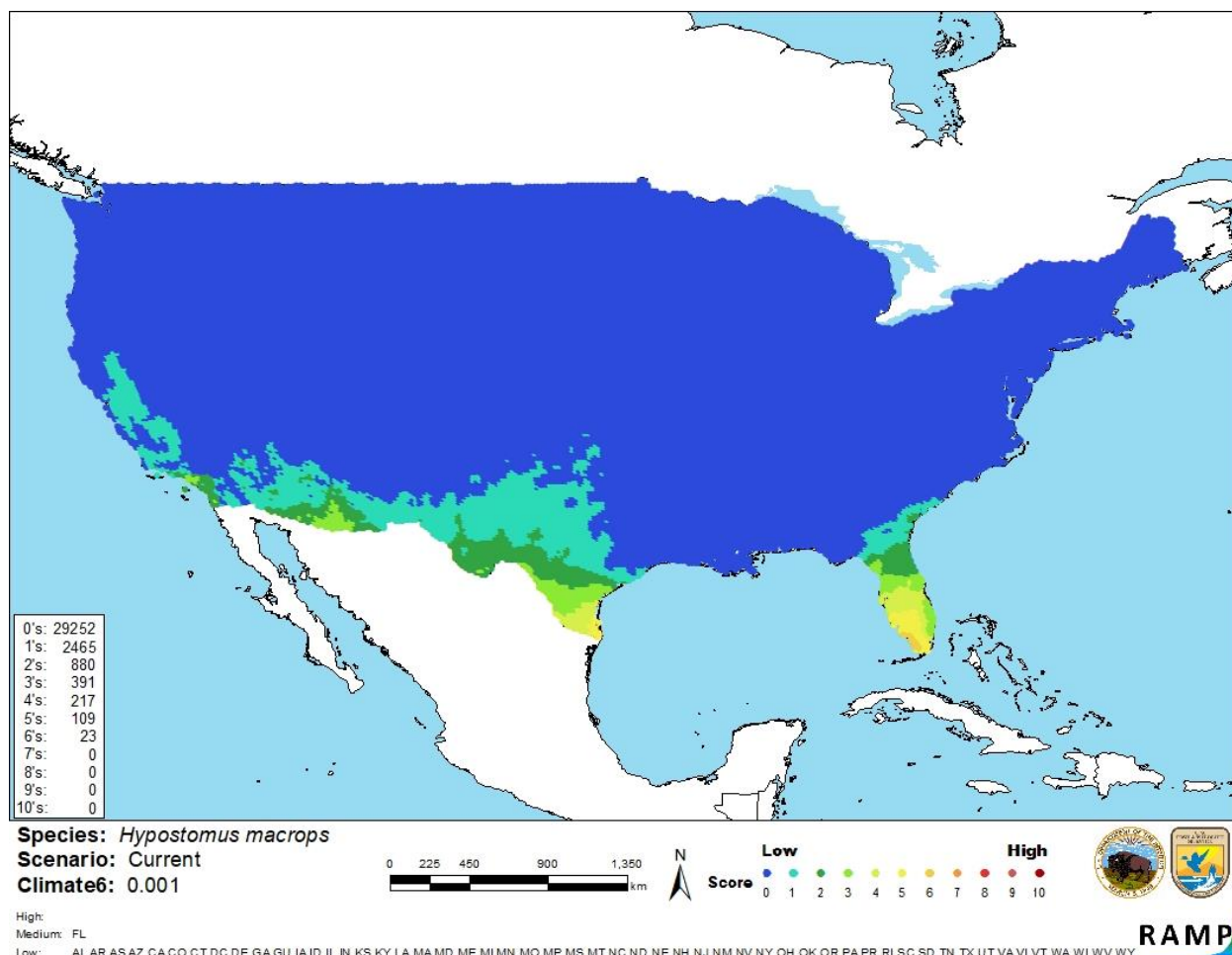
Figure 3. Map of RAMP (Sanders et al. 2018) climate matches for H. macrops in the contiguous United States based on source locations reported by GBIF Secretariat (2017). 0= Lowest match, 10= Highest match.
