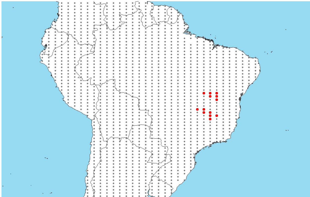
Figure 2. RAMP (Sanders et al. 2018) source map showing weather stations selected as source locations (red; Brazil) and non-source locations (gray) for H. macrops climate matching. Source locations from GBIF Secretariat (2017).
