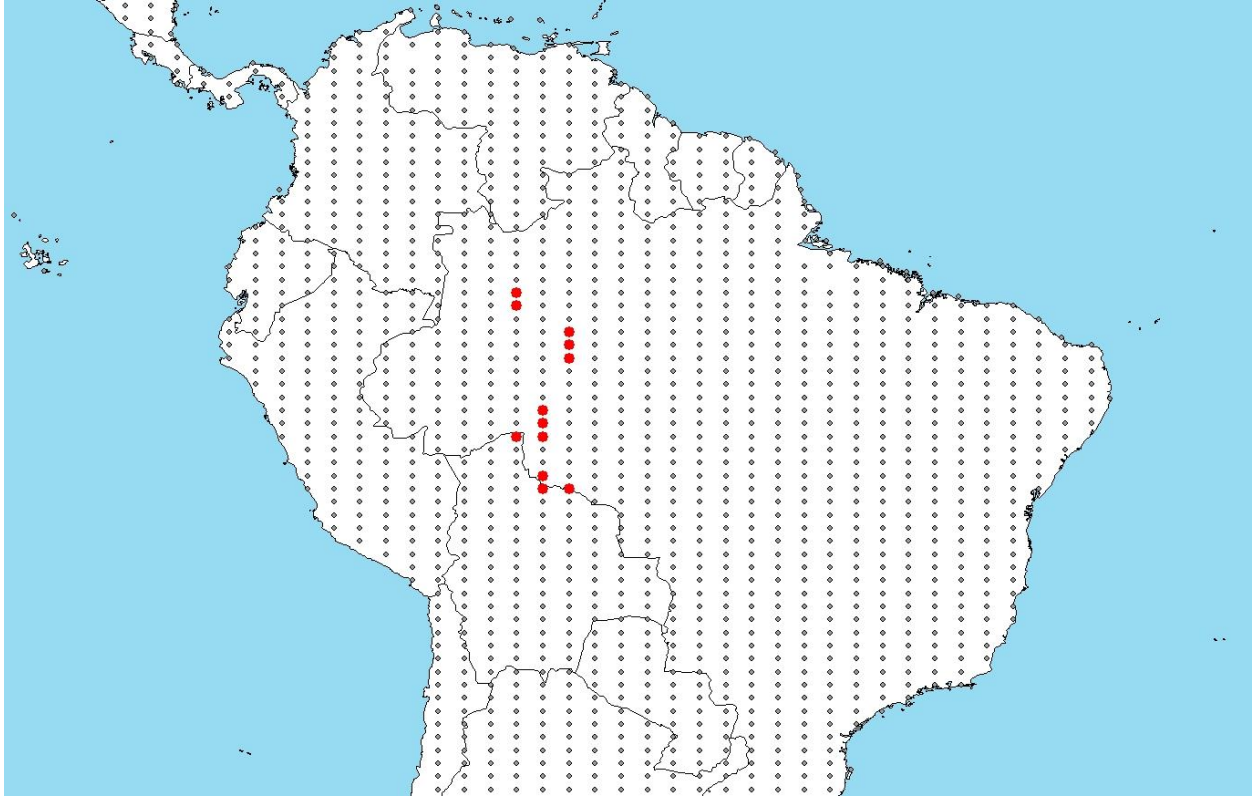
Figure 2. RAMP (Sanders et al. 2018) source map showing weather stations selected as source locations (red; Brazil, Bolivia) and non-source locations (gray) for Hypostomus hoplonites climate matching. Source locations from GBIF Secretariat (2017).
