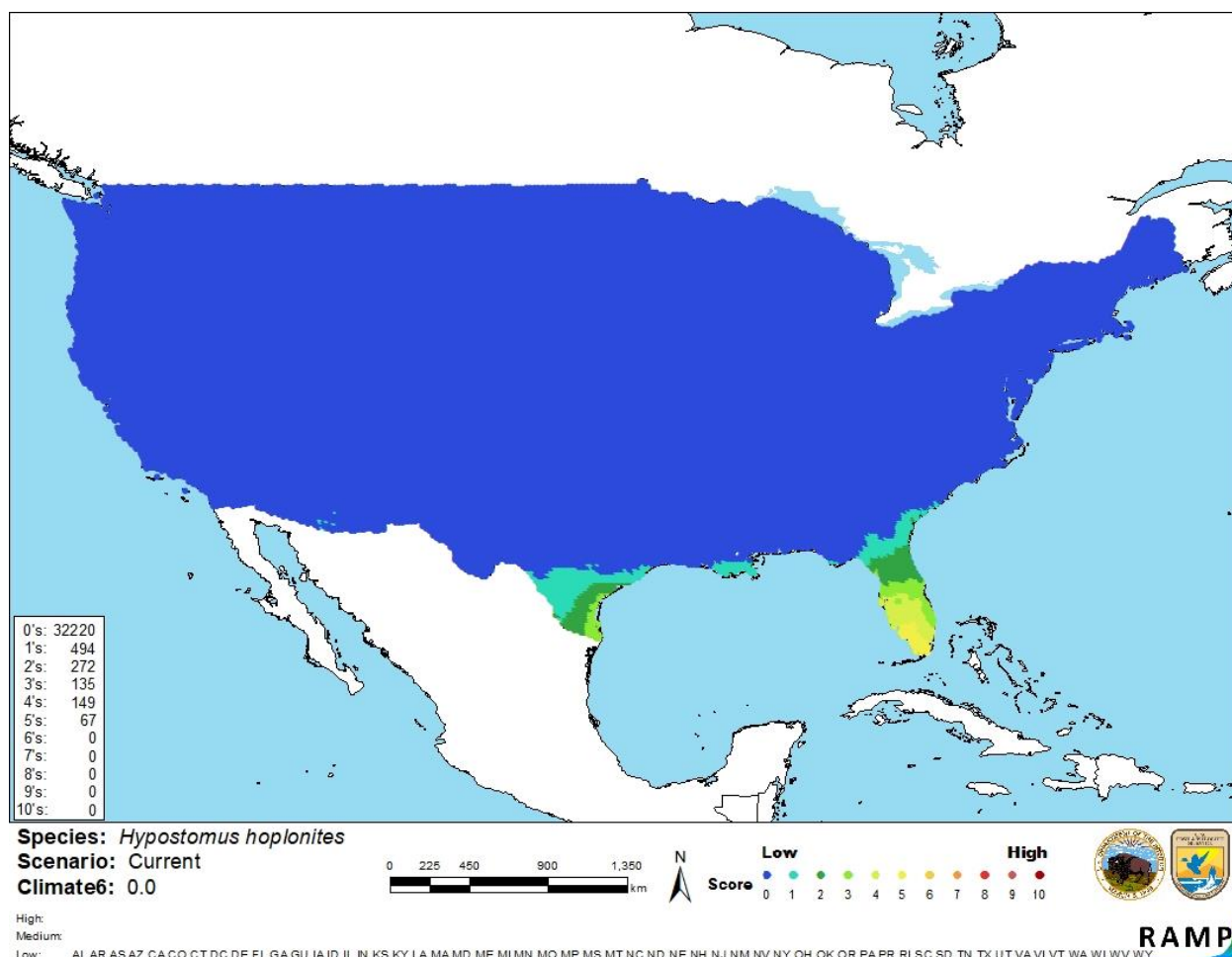
Figure 3. Map of RAMP (Sanders et al. 2018) climate matches for Hypostomus hoplonites in the contiguous United States based on source locations reported by GBIF Secretariat (2017). 0= Lowest match, 10= Highest match.
