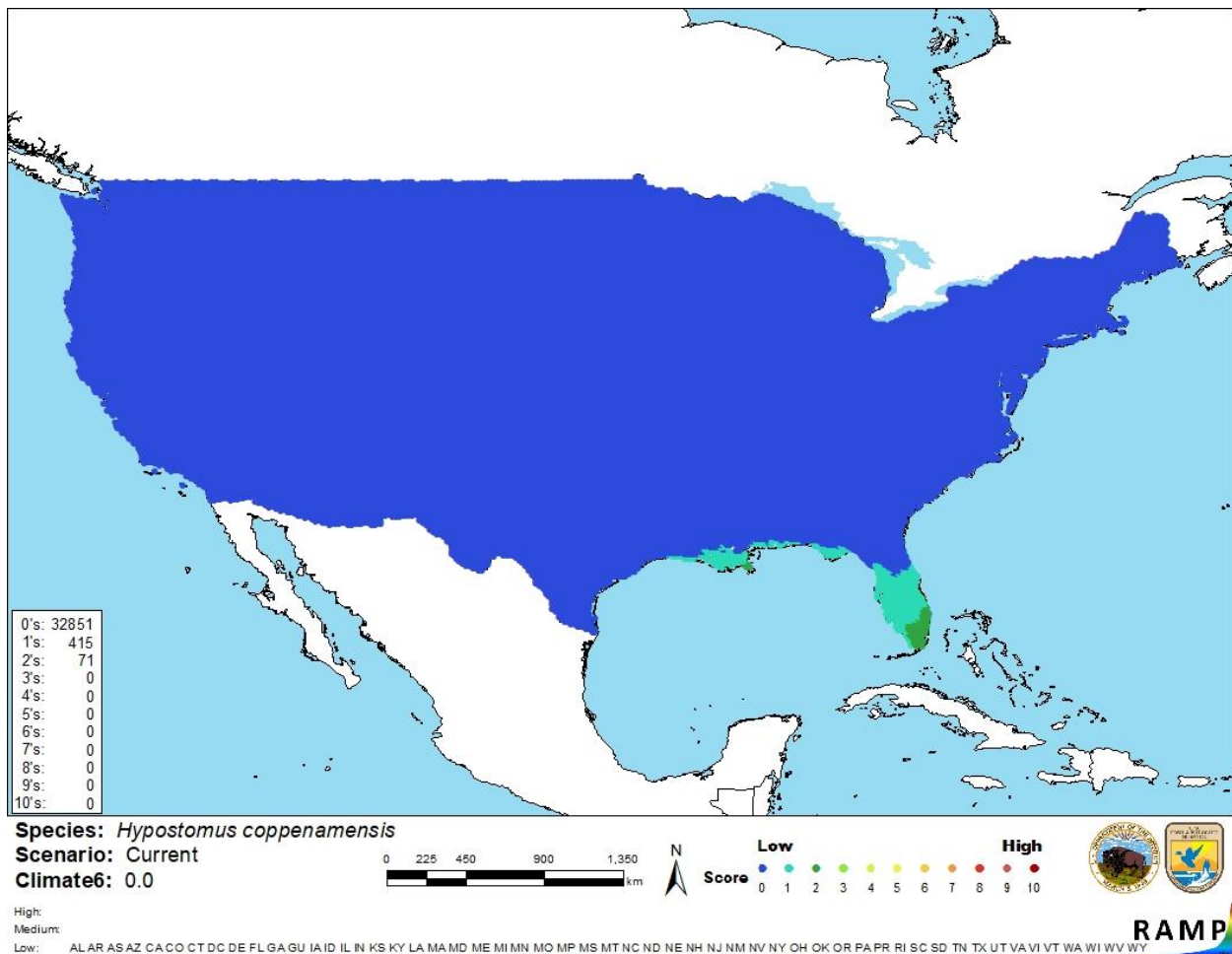
Figure 3. Map of RAMP (Sanders et al. 2018) climate matches for Hypostomus coppenamensis in the contiguous United States based on source locations reported by GBIF Secretariat (2017). Counts of climate match scores are tabulated on the left. 0= Lowest match, 10= Highest match.
