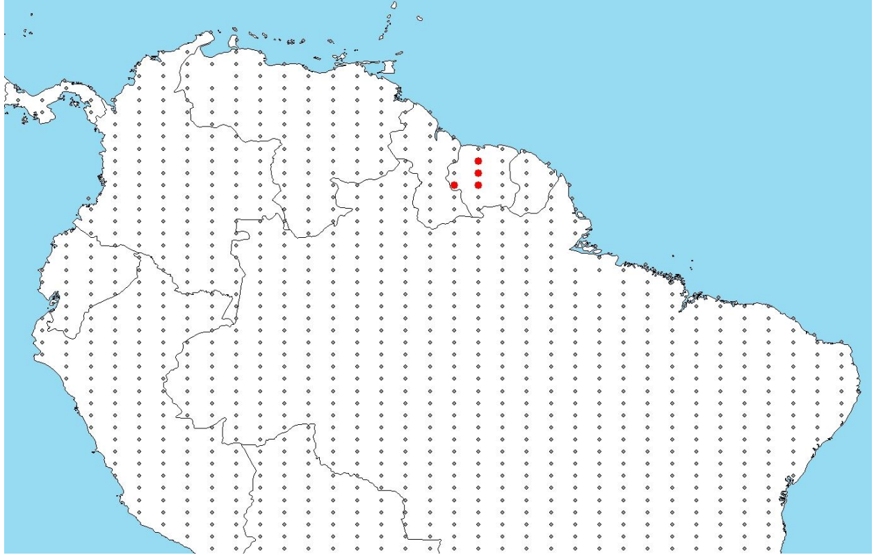
Figure 2. RAMP (Sanders et al. 2018) source map showing weather stations selected as source locations (red; Suriname) and non-source locations (gray) for Hypostomus coppenamensis climate matching. Source locations from GBIF Secretariat (2017).
