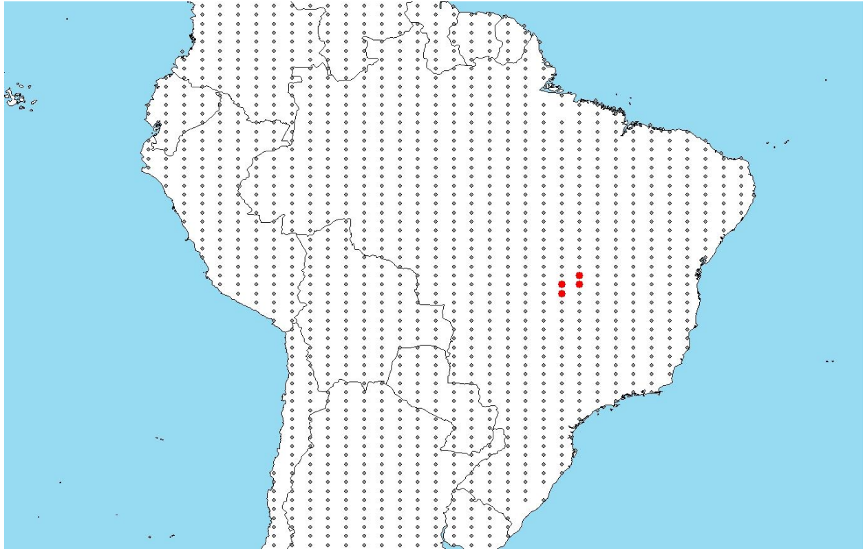
Figure 2. RAMP (Sanders et al. 2018) source map showing weather stations selected as source locations (red; Brazil) and non-source locations (gray) for H. asperatus climate matching. Source locations from GBIF Secretariat (2017).
