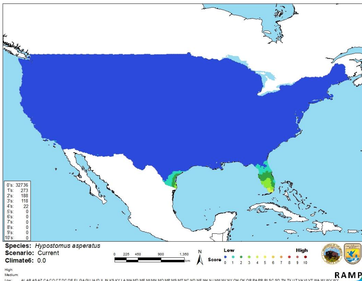
Figure 3. Map of RAMP (Sanders et al. 2018) climate matches for H. asperatus in the contiguous United States based on source locations reported by GBIF Secretariat (2017). Counts of climate match scores are tabulated on the left. 0= Lowest match, 10= Highest match.
