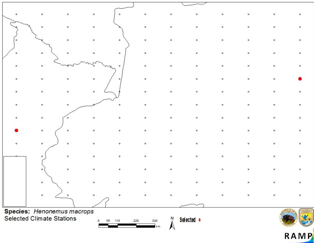
Figure 2. RAMP (Sanders et al. 2014) source map showing weather stations in northern Peru and western Brazil selected as source locations (red) and non-source locations (gray) for Henonemus macrops climate matching. Source locations from Reis et al. (2003) and GBIF (2016).
