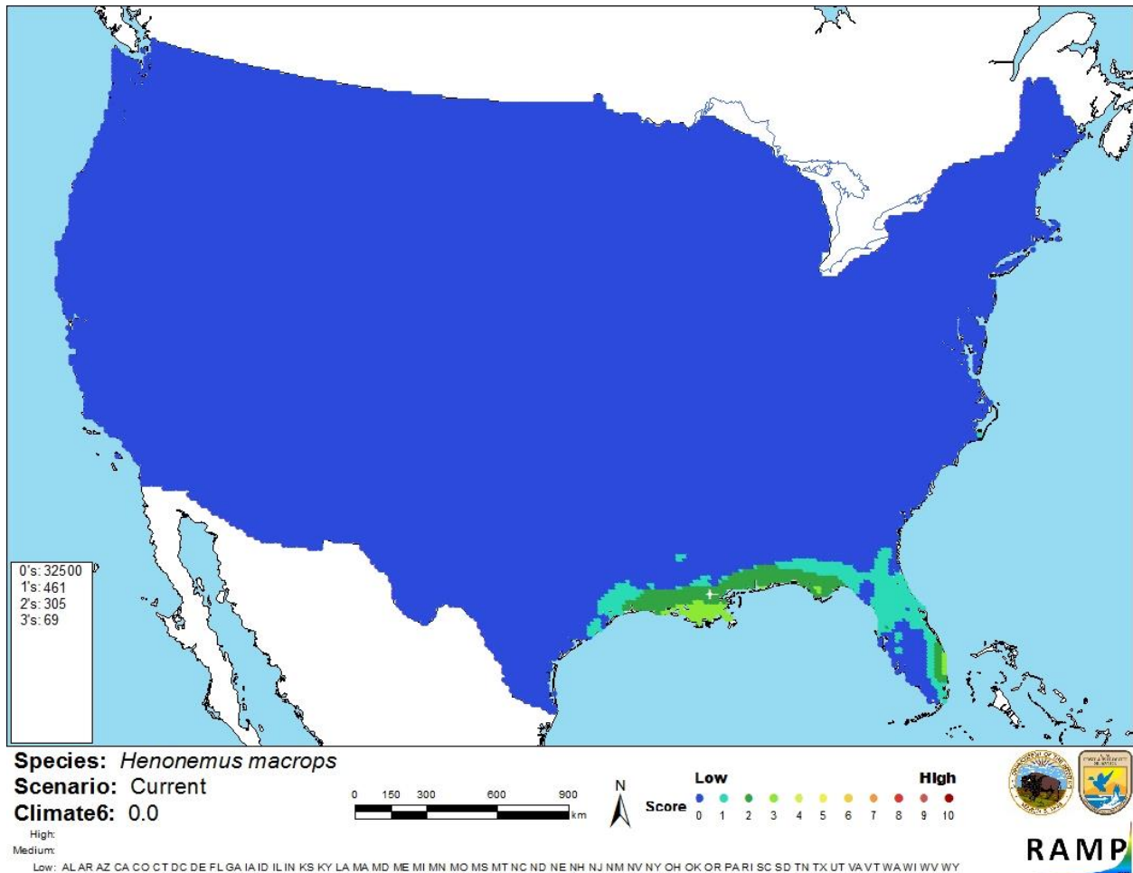
Figure 3. Map of RAMP (Sanders et al. 2014) climate matches for Henonemus macrops in the contiguous United States based on source locations reported by Reis et al. (2003) and GBIF (2016). 0= Lowest match, 10=Highest match. Counts of climate matches are tabulated on the left.
