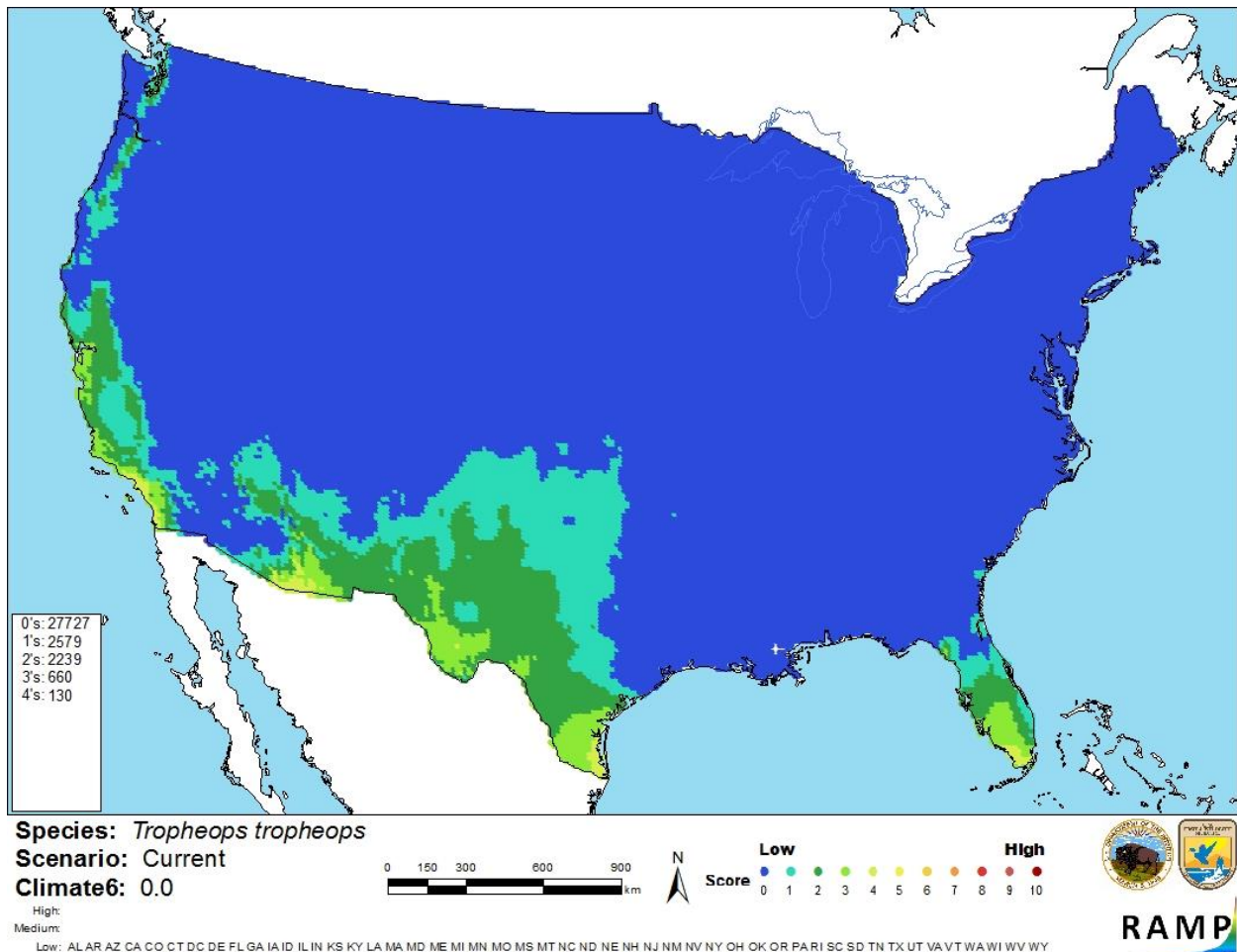
Figure 4. Map of RAMP (Sanders et al. 2014) climate matches for Tropheops tropheops in the contiguous United States based on source locations reported by GBIF Secretariat (2017). 0 = Lowest match, 10 = Highest match.
