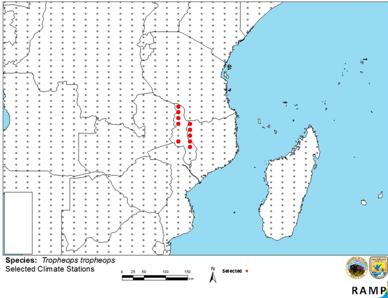
Figure 3. RAMP (Sanders et al. 2014) source map showing weather stations selected as source locations (red; Malawi, Mozambique) and non-source locations (grey) for Tropheops tropheops climate matching. Source locations from GBIF Secretariat (2017). Selected source locations are within 100 km of one or more species occurrences, and do not necessarily represent the locations of occurrences themselves.
