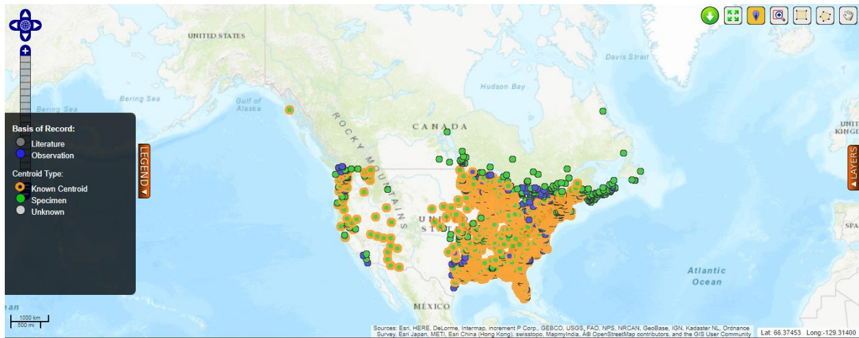
Figure 2. Known distribution of Nymphaea odorata in the United States. Map from BISON (2018). The eastern United States is within N. odorata 's native range (NatureServe 2018).
