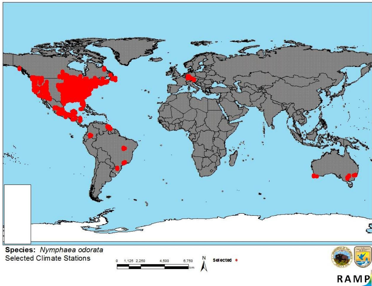
Figure 3. RAMP (Sanders et al. 2014) source map showing weather stations in North and South America, Germany, and Australia selected as source locations (red) and non-source locations (gray) for Nymphaea odorata climate matching. Source locations from BISON (2018) and GBIF Secretariat (2018). Selected source locations are within 100 km of one or more species occurrences, and do not necessarily represent the locations of occurrences themselves.
