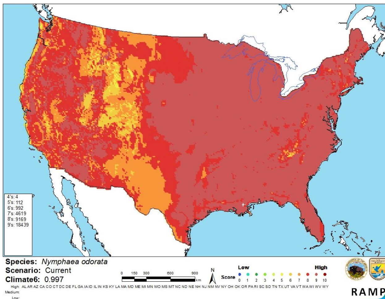
Figure 4. Map of RAMP (Sanders et al. 2014) climate matches for Nymphaea odorata in the contiguous United States based on source locations reported by BISON (2018) and GBIF Secretariat (2018). Counts of climate match are tabulated on the left. 0/Blue = Lowest match, 10/Red = Highest match.
