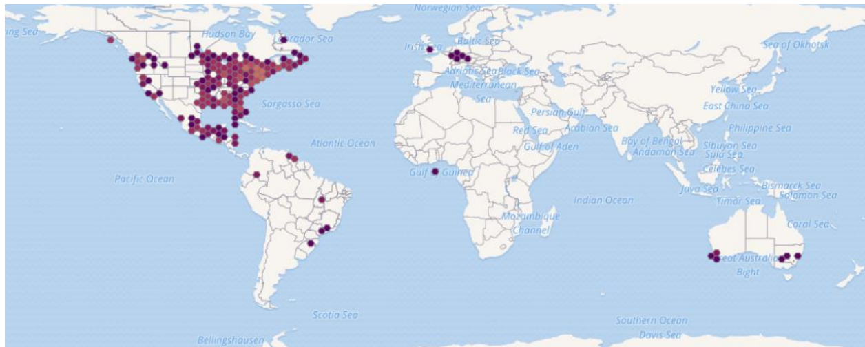
Figure 1. Known global distribution of Nymphaea odorata . Locations are in North and South America, Europe, and Australia. Map from GBIF Secretariat (2018).
