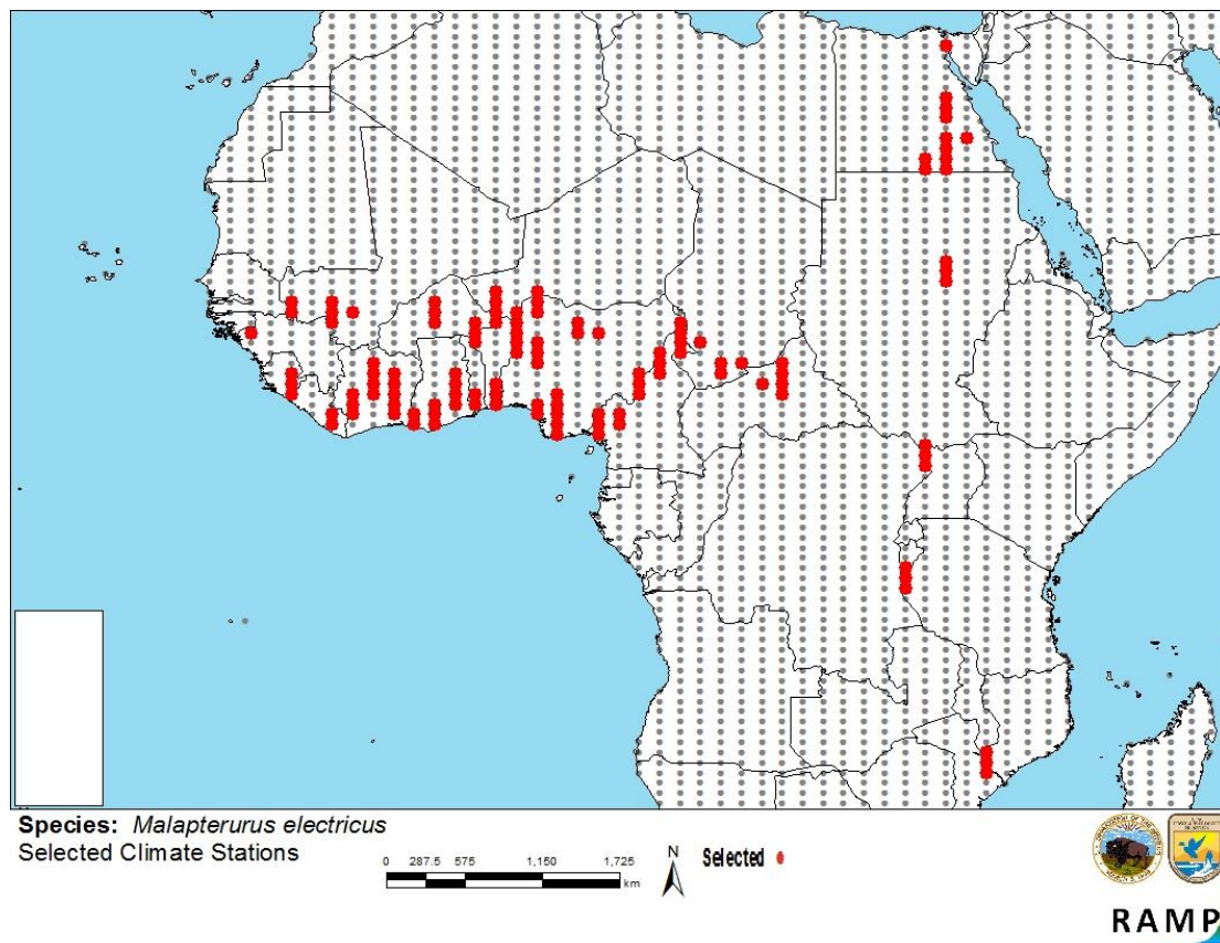
Figure 2. RAMP (Sanders et al. 2014) source map showing weather stations selected as source locations (red) and non-source locations (gray) for Malapterus electricus climate matching. Source locations from GBIF (2016); one location in the U.S. was excluded because of uncertainty over the origin and location of the specimen, and additional locations were excluded from parts or all of the following African countries because they lay outside the described native range (Figure 1): Botswana, Cameroon (southern), Democratic Republic of the Congo (southern), Egypt (Sinai Peninsula), Equatorial Guinea, Gabon, Guinea-Bissau, Mozambique, Republic of the Congo, Senegal, and Zimbabwe.
