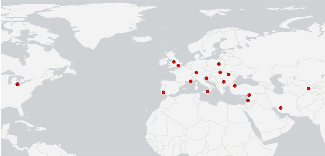
Figure 2. Additional known distribution of Cyclops abyssorum divergens . Observations are reported from Lake Erie in North America, Europe, and western Asia. Map from Esri (2022) based on locations described by Hołyńska (2008) and Connolly et al. (2022).
