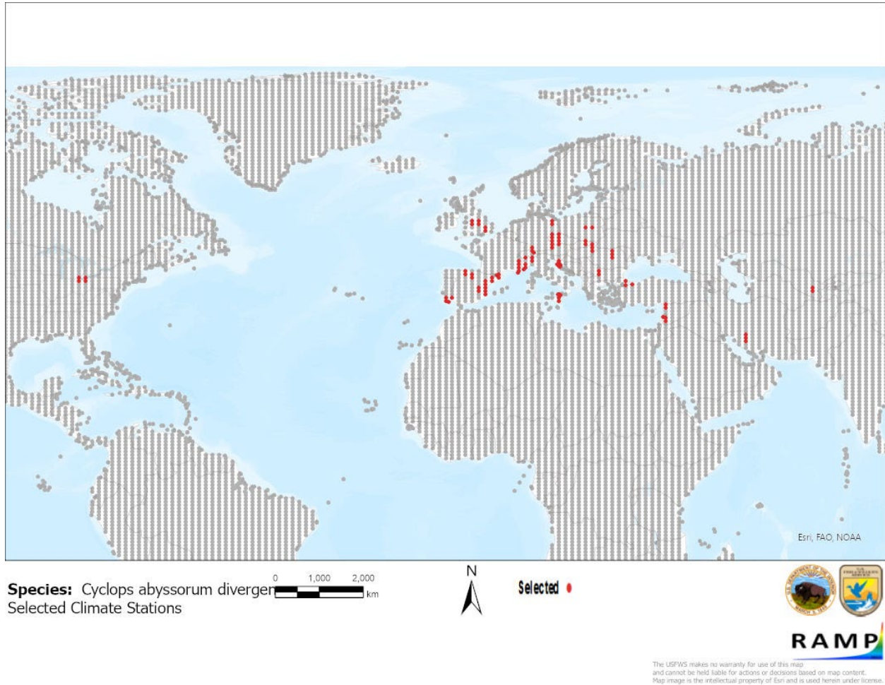
Figure 4. RAMP (Sanders et al. 2021) source map showing weather stations in the northern hemisphere selected as source locations (red; United States, Canada, Portugal, Spain, France, United Kingdom, Switzerland, Italy, Germany, Austria, Poland, Czechia, Croatia, Slovakia, Hungary, Bulgaria, Romania, Turkey, Lebanon, Syria, Iran, and Uzbekistan) and non-source locations (gray) for Cyclops abyssorum divergens climate matching. Source locations from GBIF Secretariat (2022), Hołyńska (2008), and Connolly et al. (2022). Selected source locations are within 100 km of one or more species occurrences, and do not necessarily represent the locations of occurrences themselves.
