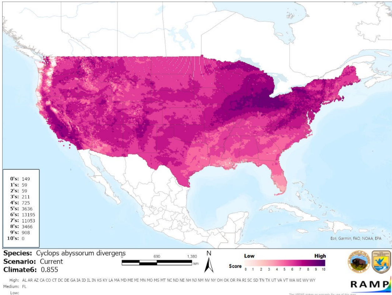
Figure 5. Map of RAMP (Sanders et al. 2021) climate matches for Cyclops abyssorum divergens in the contiguous United States based on source locations reported by GBIF Secretariat (2022), Hołyńska (2008), and Connolly et al. (2022). Counts of climate match scores are tabulated on the left. 0/Pale Pink = Lowest match, 10/Dark Purple = Highest match.
