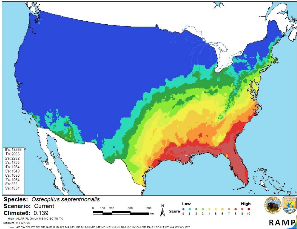
Figure 4. Map of RAMP (Sanders et al. 2014) climate matches for Osteopilus septentrionalis in the contiguous United States based on source locations reported by GBIF Secretariat (2018) and Somma et al. (2018). Counts of climate match scores are tabulated on the left. 0 = Lowest match, 10 = Highest match.
