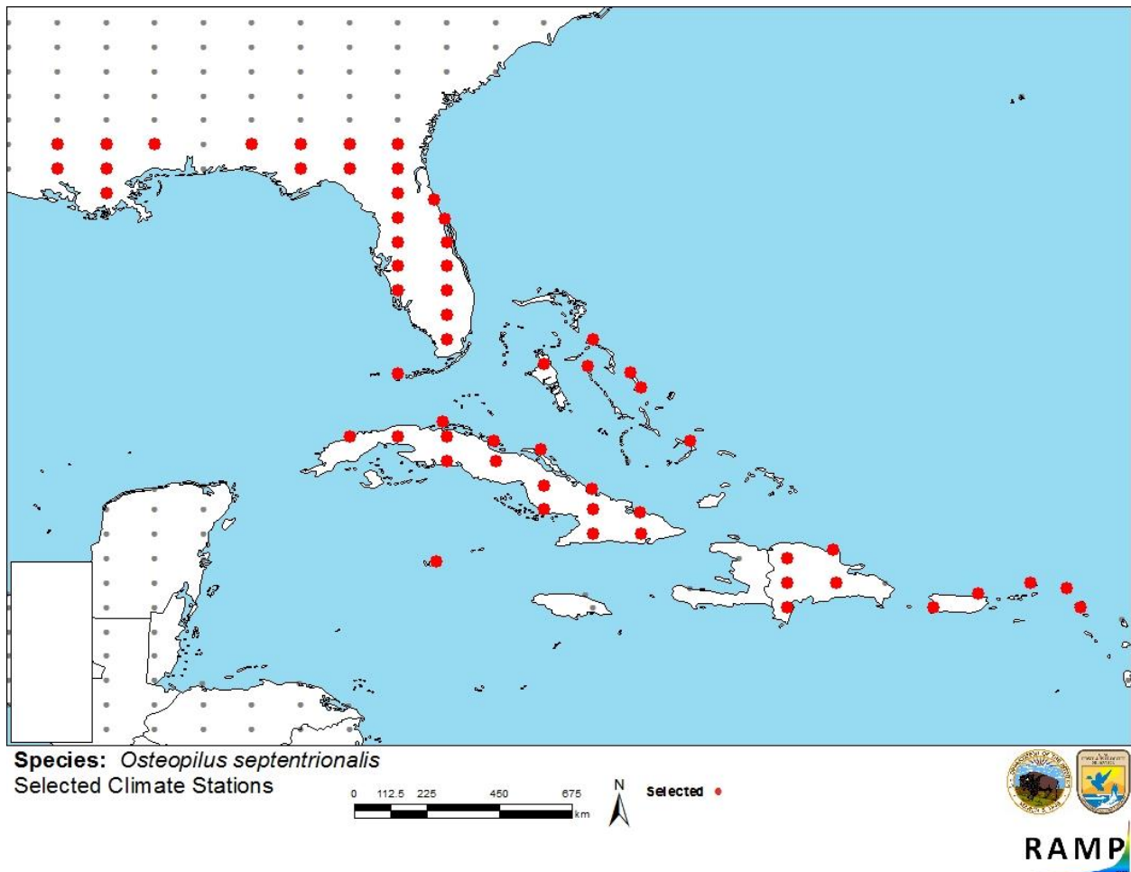
Figure 3. RAMP (Sanders et al. 2014) source map showing weather stations in the southeastern United States and Caribbean selected as source locations (red) and non-source locations (gray) for Osteopilus septentrionalis climate matching. Source locations from GBIF Secretariat (2018) and Somma et al. (2018).
