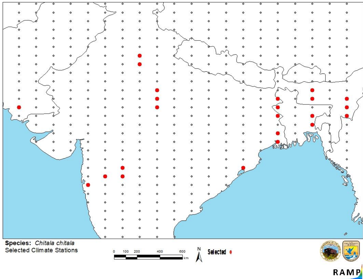
Figure 2. RAMP (Sanders et al. 2018) source map showing weather stations in Bangladesh, India, Nepal, and Pakistan selected as source locations (red) and non-source locations (gray) for Chitala chitala climate matching. Source locations from GBIF Secretariat (2019). Selected source locations are within 100 km of one or more species occurrences, and do not necessarily represent the locations of occurrences themselves.
