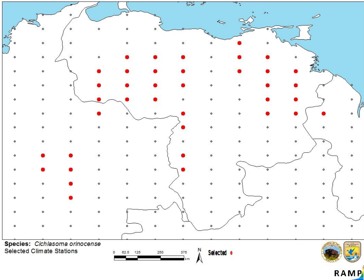
Figure 2. RAMP (Sanders et al. 2018) source map showing weather stations in South America selected as source locations (red; Columbia, Guyana, and Venezuela) and non-source locations (gray) for Cichlasoma orinocense climate matching. Source locations from GBIF Secretariat (2018). Selected source locations are within 100 km of one or more species occurrences, and do not necessarily represent the locations of occurrences themselves.
