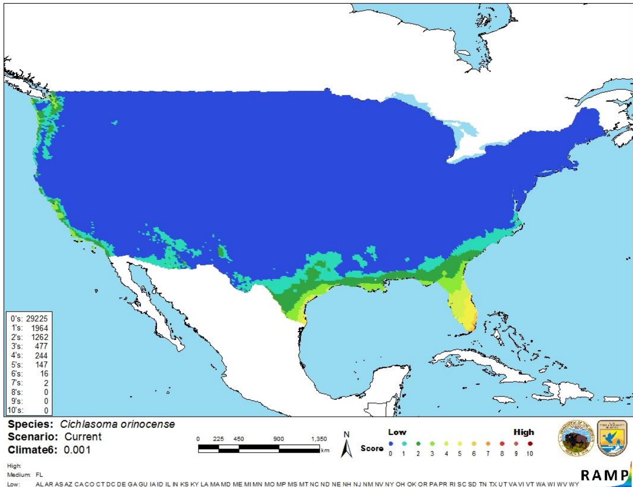
Figure 3. Map of RAMP (Sanders et al. 2018) climate matches for Cichlasoma orinocense in the contiguous United States based on source locations reported from GBIF Secretariat (2018). 0 = Lowest match, 10 = Highest match.
