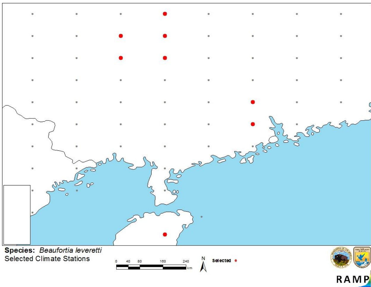
Figure 2. RAMP (Sanders et al. 2014) source map showing weather stations selected as source locations (red; China) and non-source locations (gray) for Beaufortia leveretti climate matching. Source locations from GBIF Secretariat (2014).
