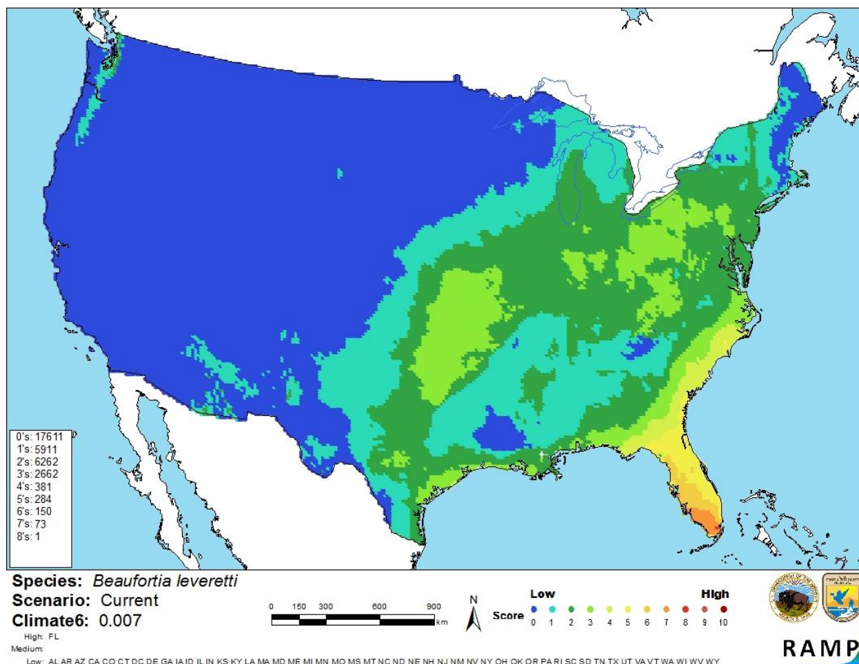
Figure 3. Map of RAMP (Sanders et al. 2014) climate matches for Beaufortia leveretti in the contiguous United States based on source locations reported by GBIF Secretariat (2014). 0 = Lowest match, 10 = Highest match. Counts of climate match scores are tabulated on the left side of the map.
