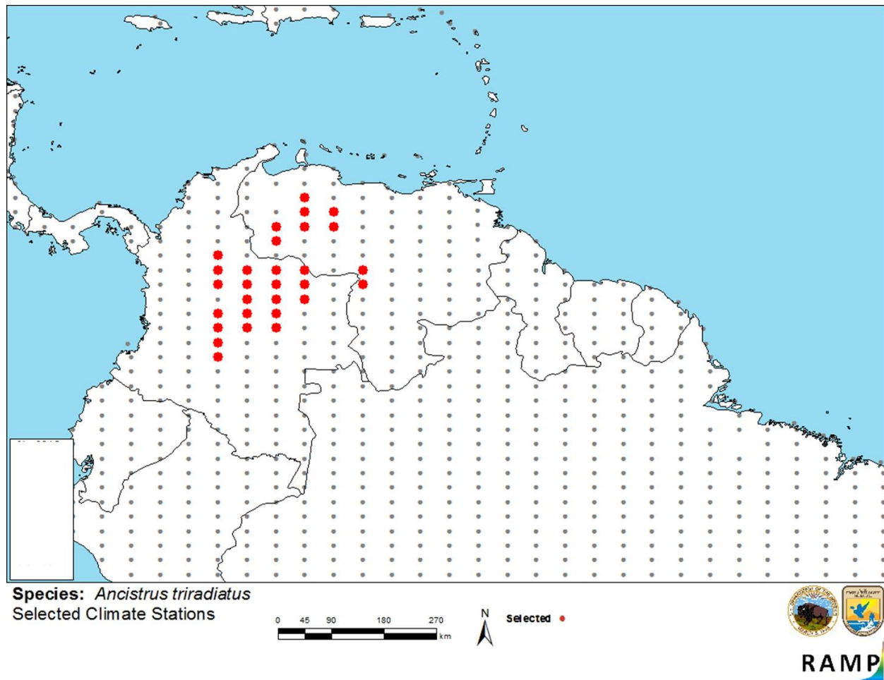
Figure 2. RAMP (Sanders et al. 2014) source map showing weather stations in Colombia and Venezuela selected as source locations (red) and non-source locations (grey) for Ancistrus triradiatus climate matching. Source locations from GBIF Secretariat (2015).
