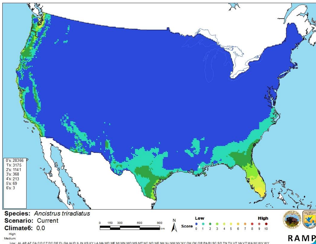
Figure 3. Map of RAMP (Sanders et al. 2014) climate matches for Ancistrus triradiatus in the contiguous United States based on source locations reported by GBIF Secretariat (2015). 0 = Lowest match, 10 = Highest match.
