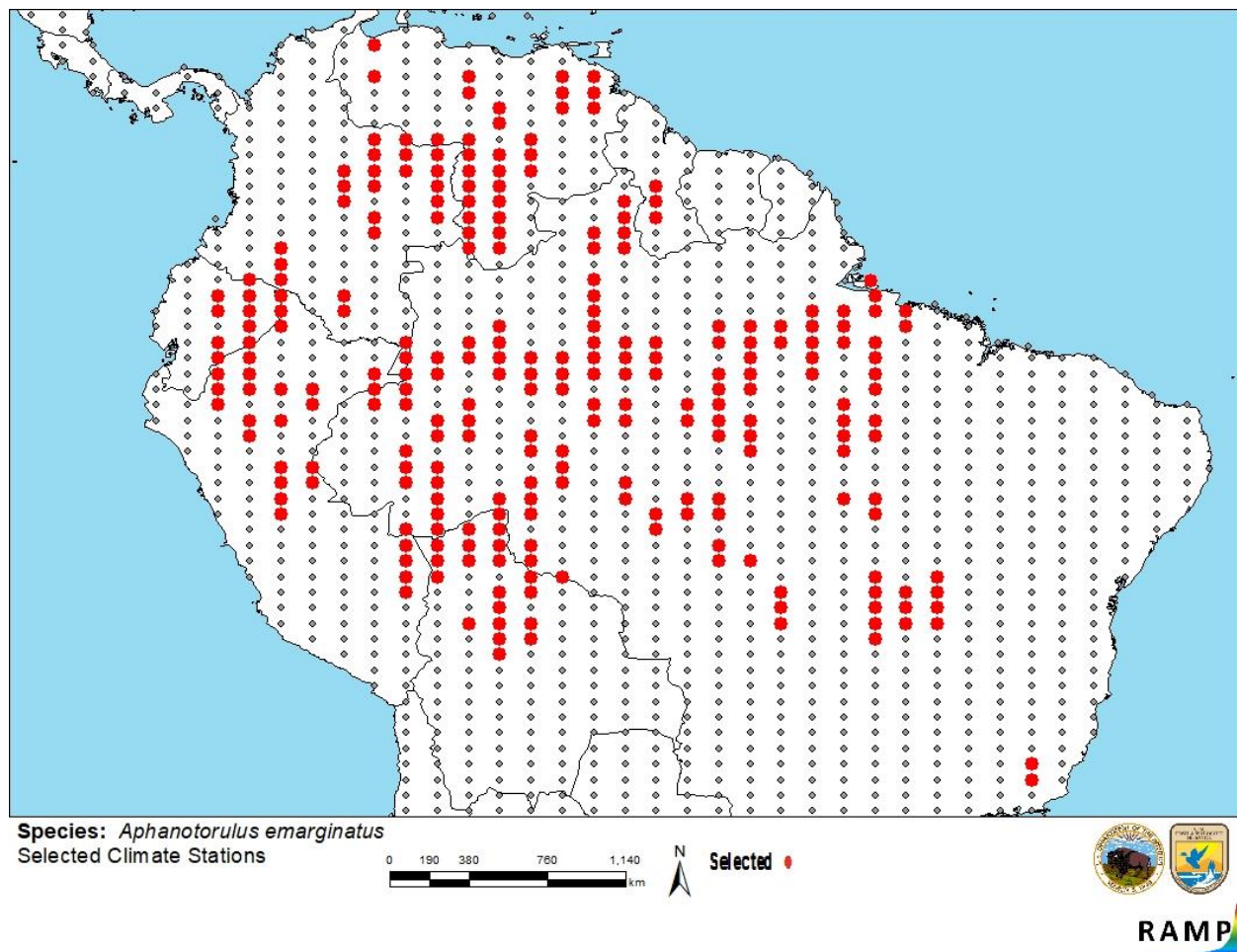
Figure 3. RAMP (Sanders et al. 2018) source map showing weather stations in South America selected as source locations (red; Colombia, Venezuela, Suriname, Ecuador, Peru, Bolivia, and Brazil) and non-source locations (gray) for Aphanotorulus emarginatus climate matching. Source locations from GBIF Secretariat (2019a, b). Selected source locations are within 100 km of one or more species occurrences, and do not necessarily represent the locations of occurrences themselves.
