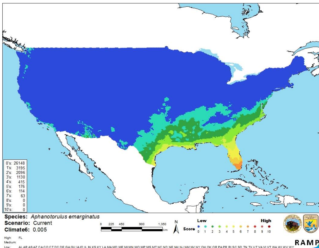
Figure 4. Map of RAMP (Sanders et al. 2018) climate matches for Aphanotorulus emarginatus in the contiguous United States based on source locations reported by GBIF Secretariat (2019a, b). Counts of climate match scores are tabulated on the left. 0 = Lowest match, 10 = Highest match.
