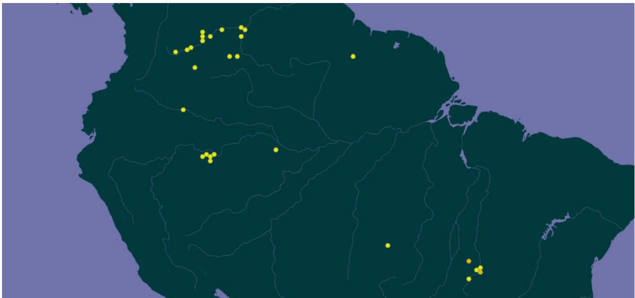
Figure 1. Known global distribution of Aphanotorulus emarginatus . Locations are in Bolivia, Brazil and Columbia. Map from GBIF Secretariat (2019a).
