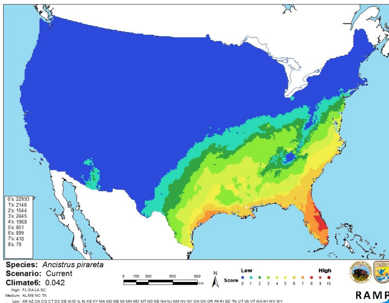
Figure 3. Map of RAMP (Sanders et al. 2014) climate matches for Ancistrus pirareta in the contiguous United States based on source locations reported by GBIF (2016). 0=Lowest match, 10=Highest match. Counts of climate match scores are tabulated on the left.
