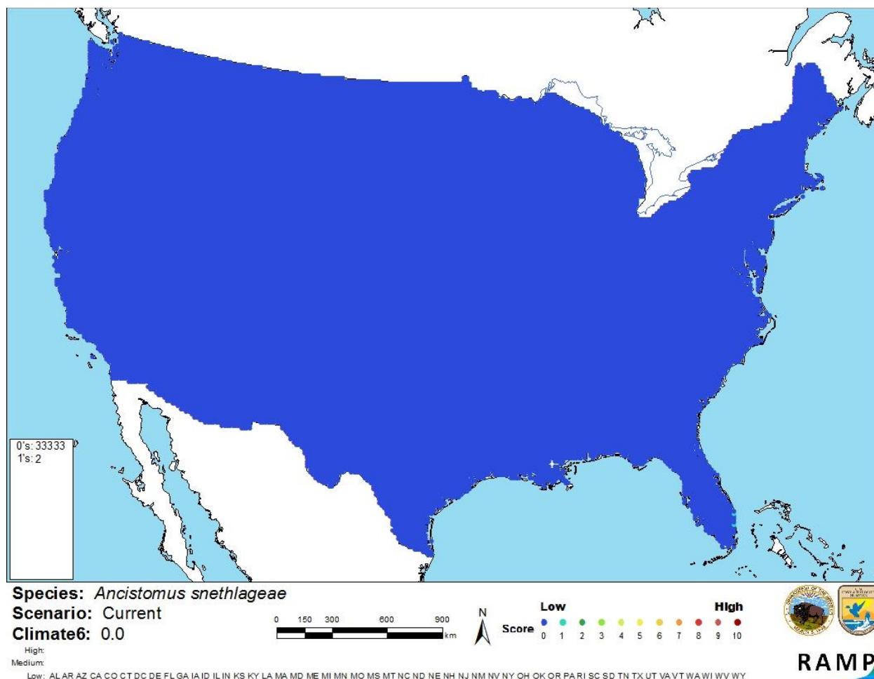
Figure 3. Map of RAMP (Sanders et al. 2014) climate matches for Ancistomus snethlageae in the contiguous United States based on source locations reported by GBIF Secretariat (2017). 0=Lowest match, 10=Highest match.
