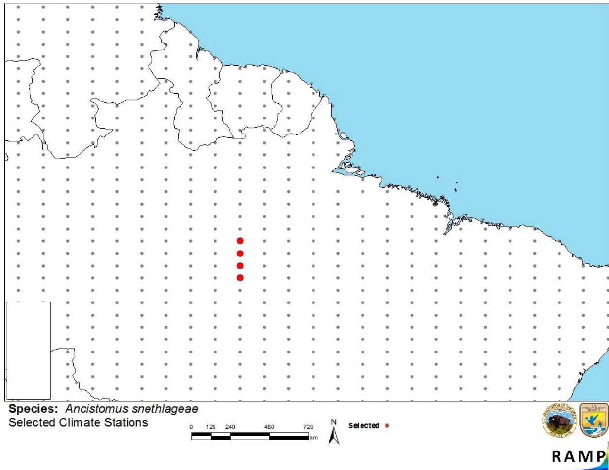
Figure 2. RAMP (Sanders et al. 2014) source map showing weather stations selected as source locations (red; Brazil) and non-source locations (gray) for Ancistomus snethlageae climate matching. Source locations from GBIF Secretariat (2017).
