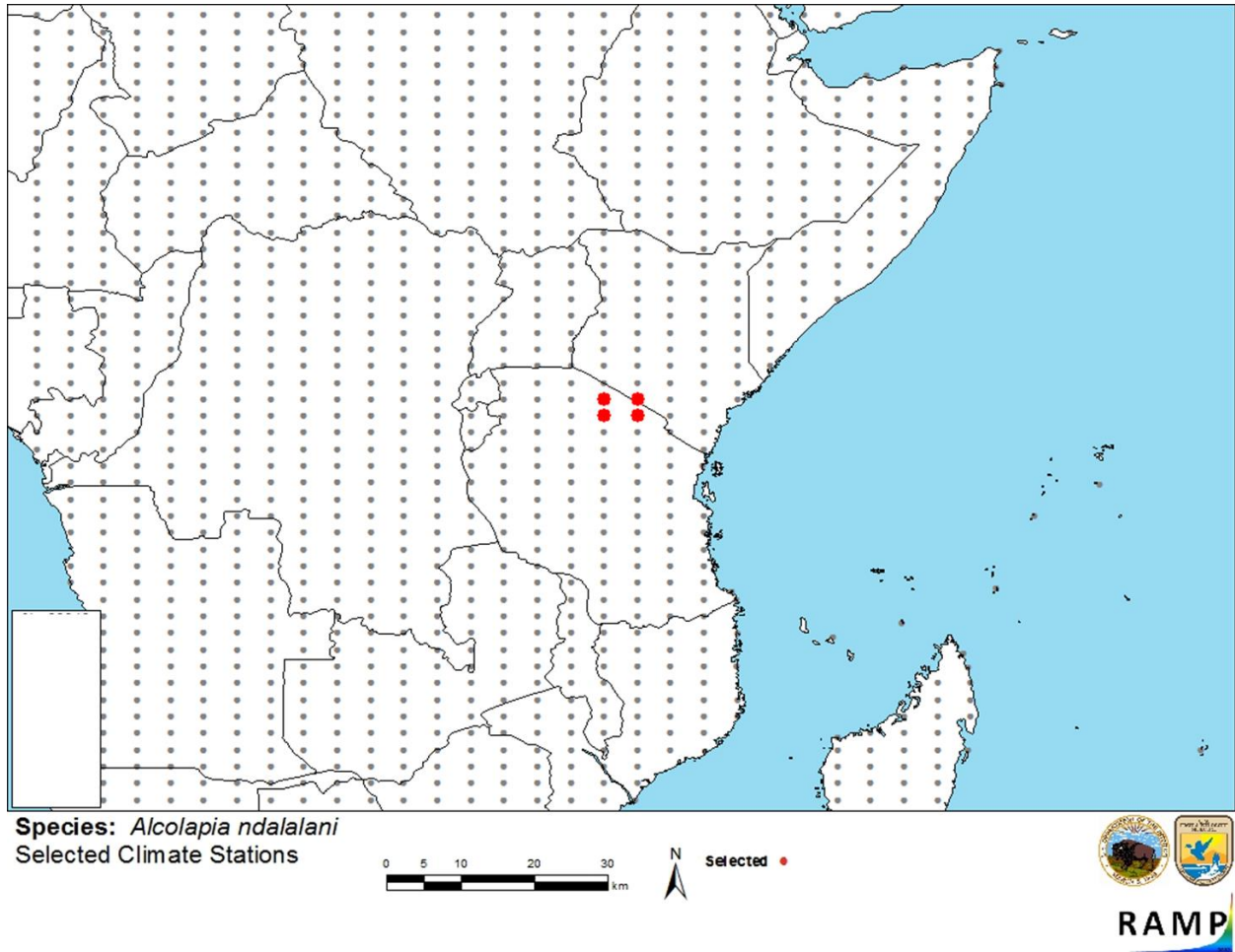
Figure 2. RAMP (Sanders et al. 2014) source map showing weather stations selected as source locations (red; Tanzania, Kenya) and non-source locations (grey) for Alcolapia ndalalani climate matching. Source locations from GBIF Secretariat (2017).
