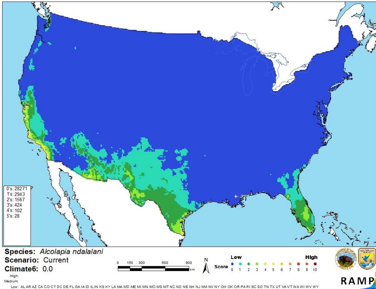
Figure 3. Map from RAMP (Sanders et al. 2014) of a current climate match for Alcolapia ndalalani in the contiguous United States based on source locations reported by GBIF Secretariat (2017). 0 = Lowest match, 10 = Highest match. Counts of climate match scores are tabulated on the left.
