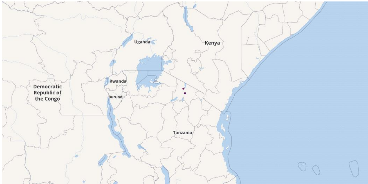
Figure 1. Known global distribution of Alcolapia ndalalani in northern Tanzania. Map from GBIF Secretariat (2017).
