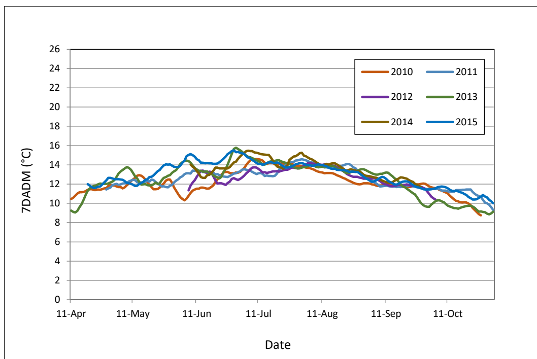
Figure 22. Seven-day averages of daily maximum water temperatures (7-DADM) in Whychus Creek near the mouth (RM 0.25) during the irrigation season. Source: UDMC 2016.
